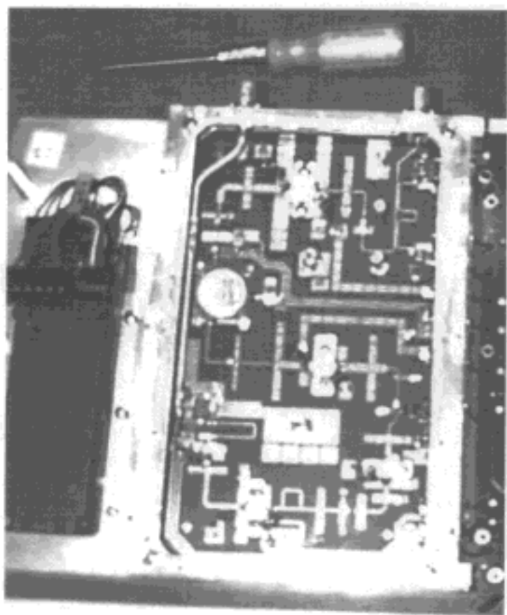
Transmitter amplifier chain
