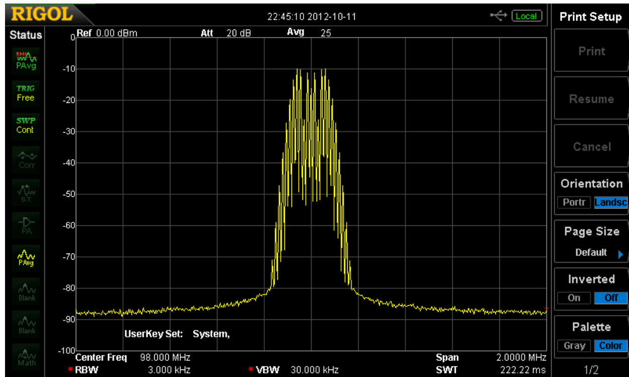
Figure 3, Occupied Bandwidth 15 kHz Left-Only
