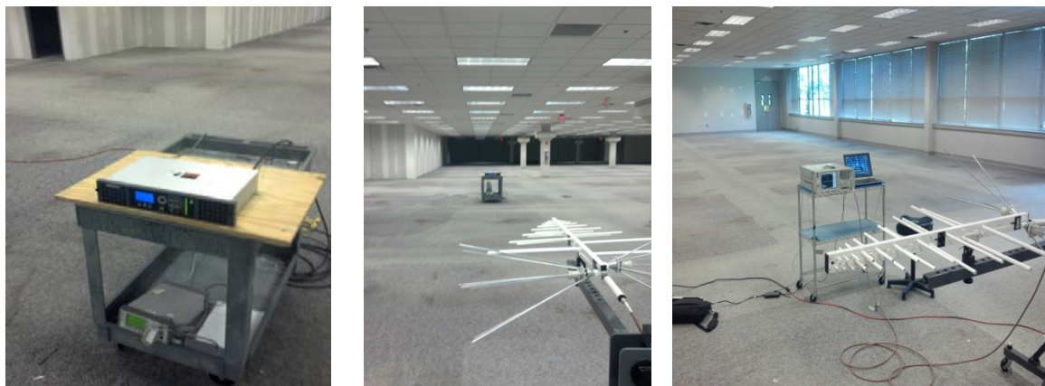
Figure 7, Transmitter under test/Test Setup
