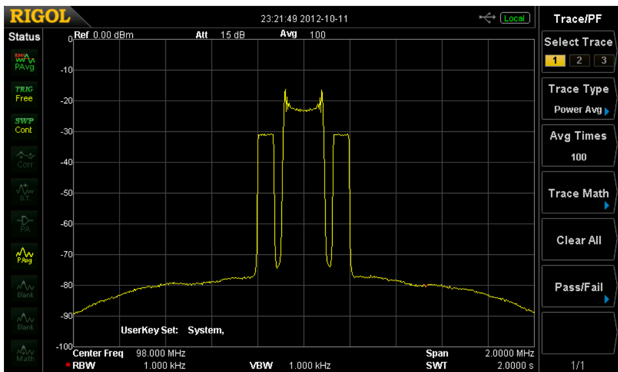
Figure 5, Occupied Bandwidth FM+HD
