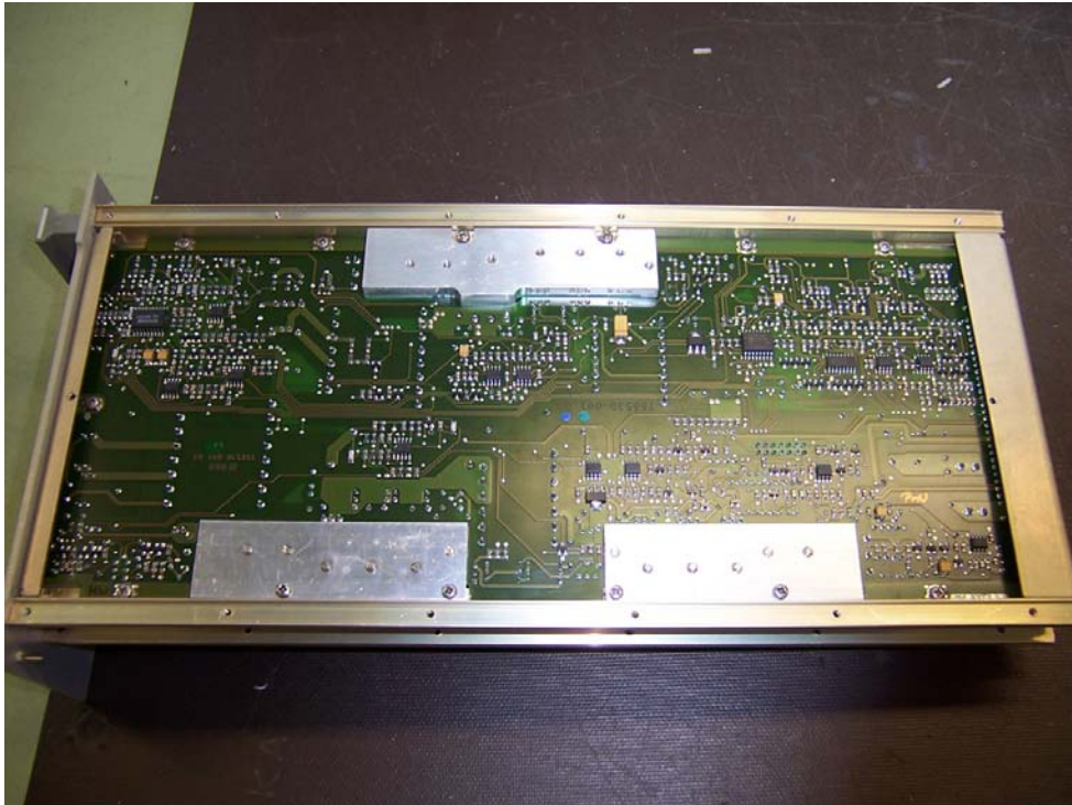
5) Frequency Processing FAB 662 977-032-003
