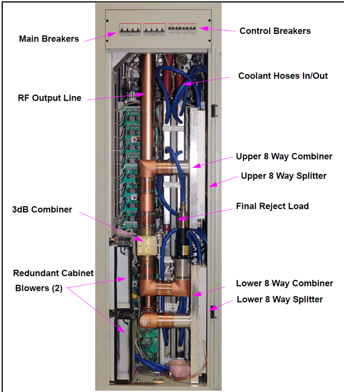
ULX Rear View, Door Removed
