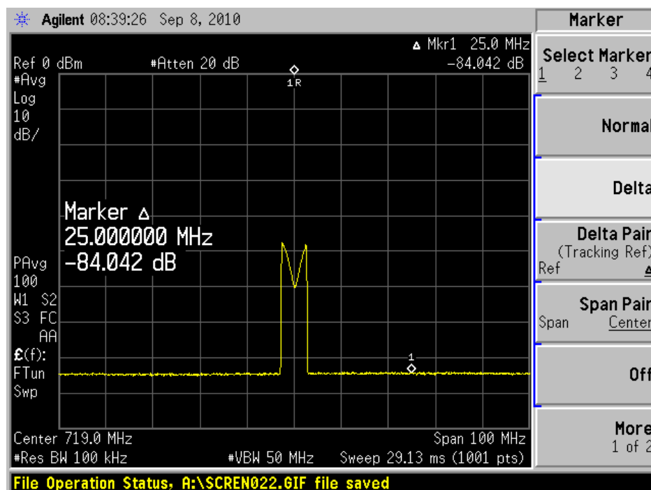
Figure 17, Transmitter Output, with Notch, With marker at 744 MHz
