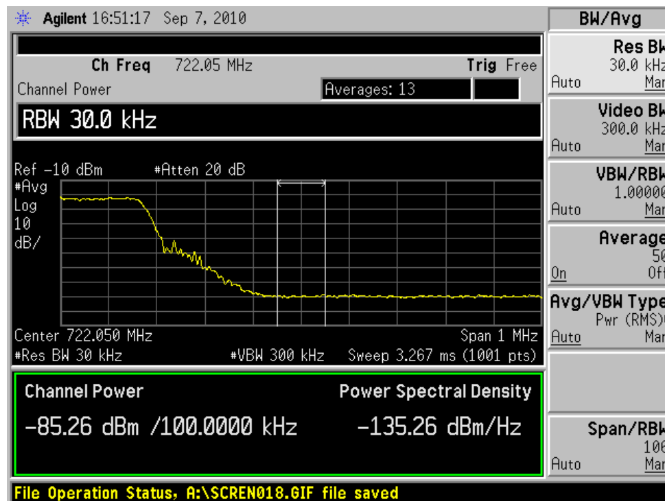
Figure 13 Upper Adjacent Channel Power
