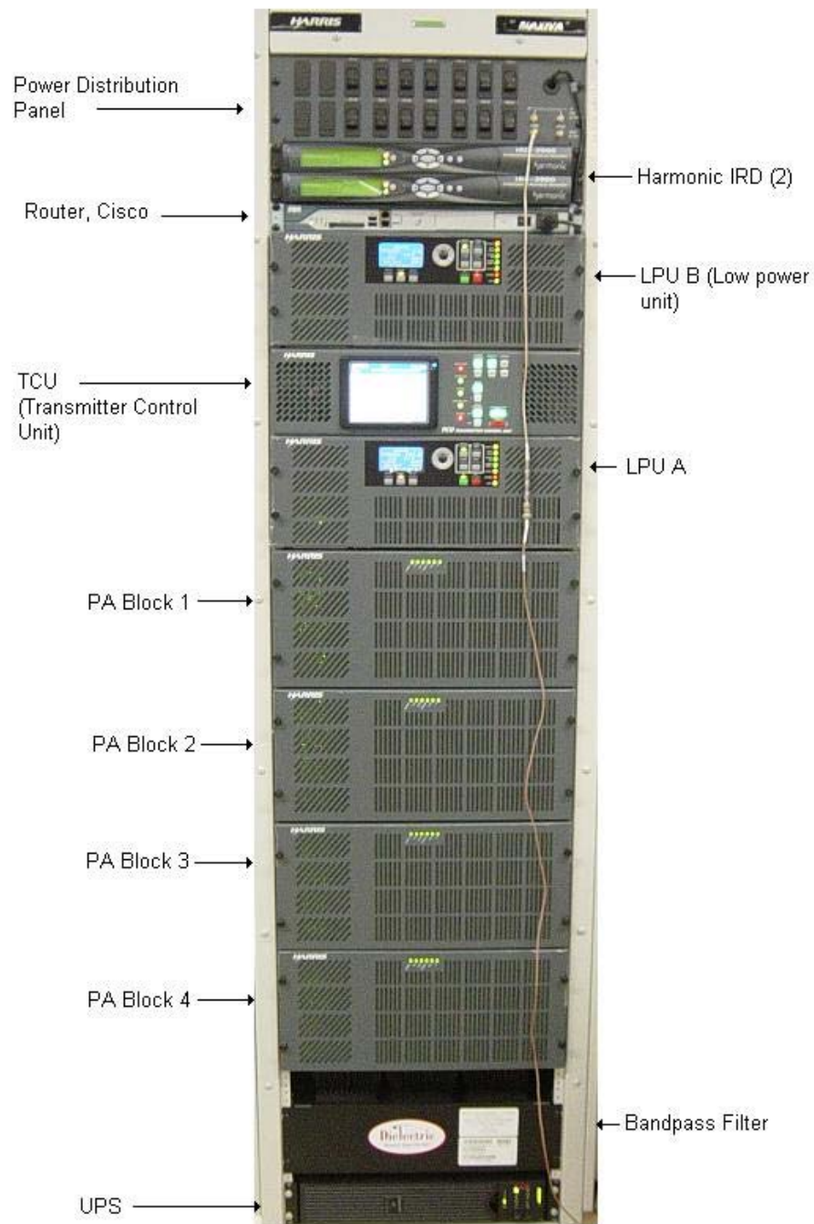
Figure 3, UAX Front View
