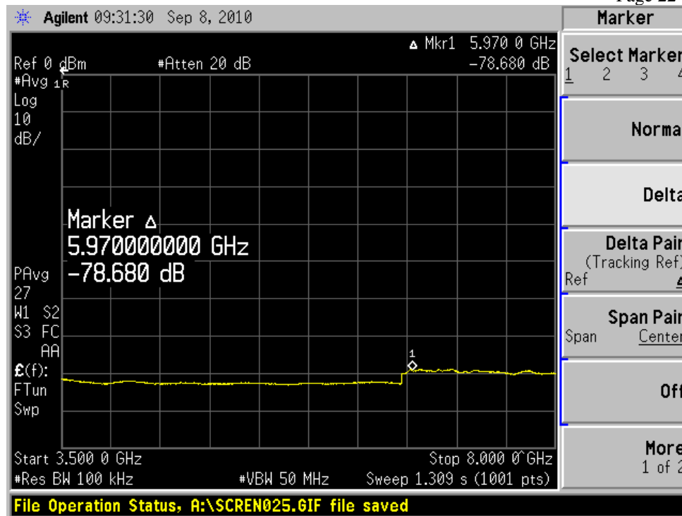
Figure 20, 3.5 GHz to 8 GHz
