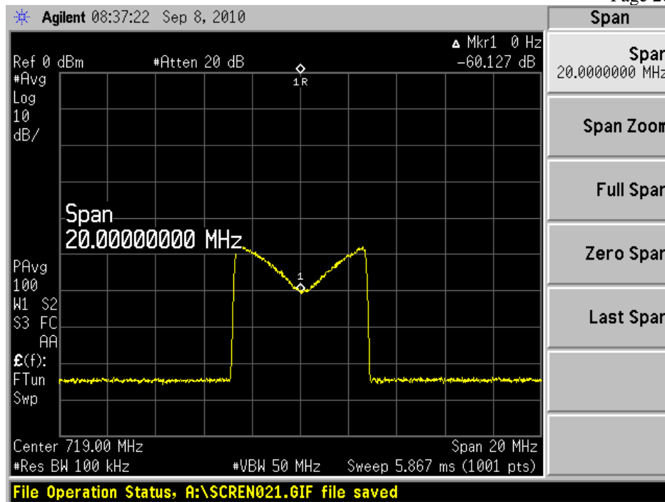
Figure 16, Transmitter Output with Carrier Notch Filter
