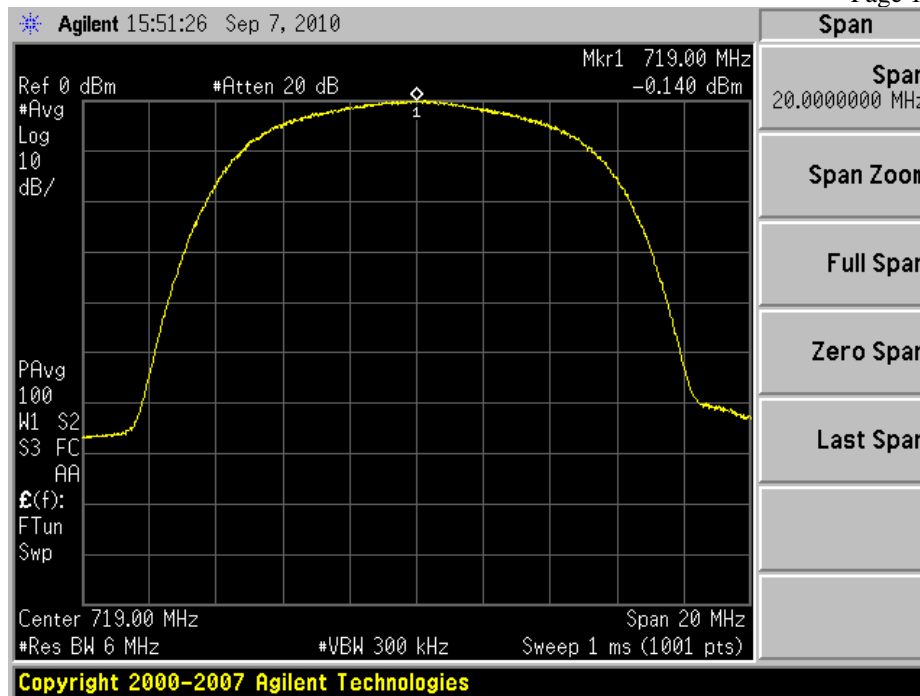
Figure 14, Transmitter Output in 6 MHz BW
