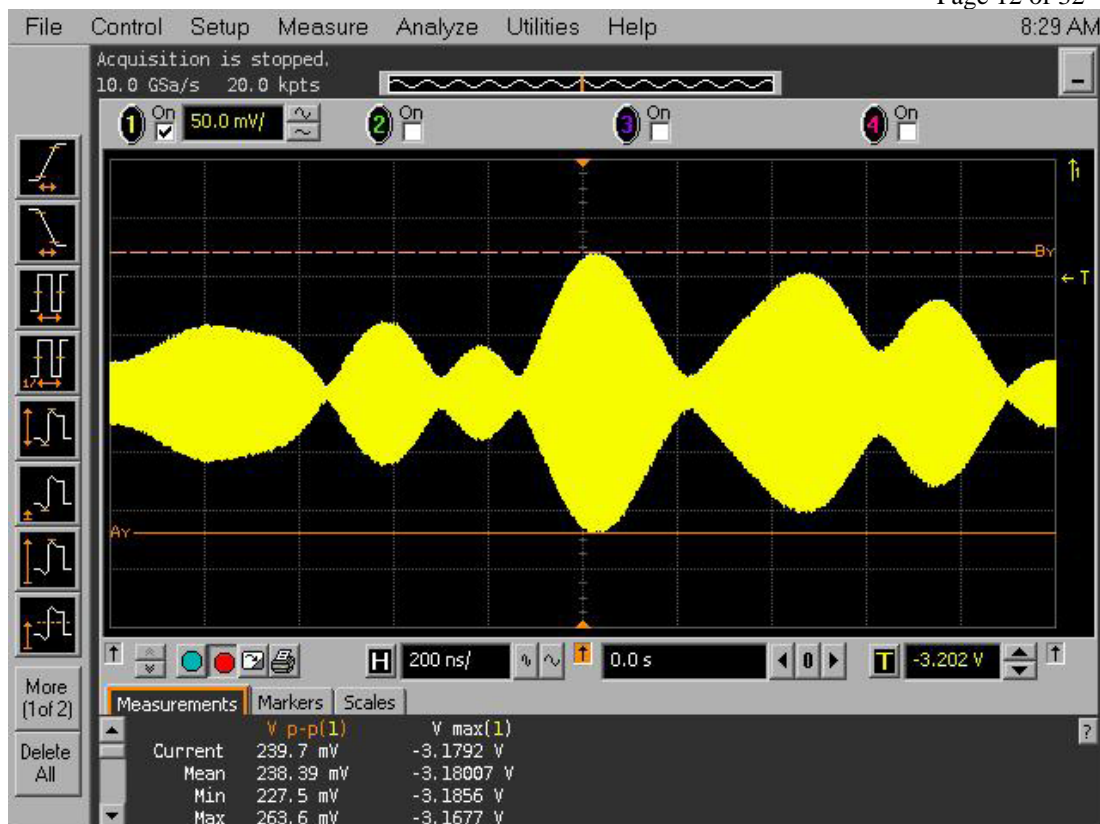
Figure 7, FLO Signal Time Domain Plot
