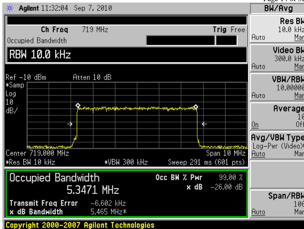
Figure 9, Occupied Bandwidth at System Output
