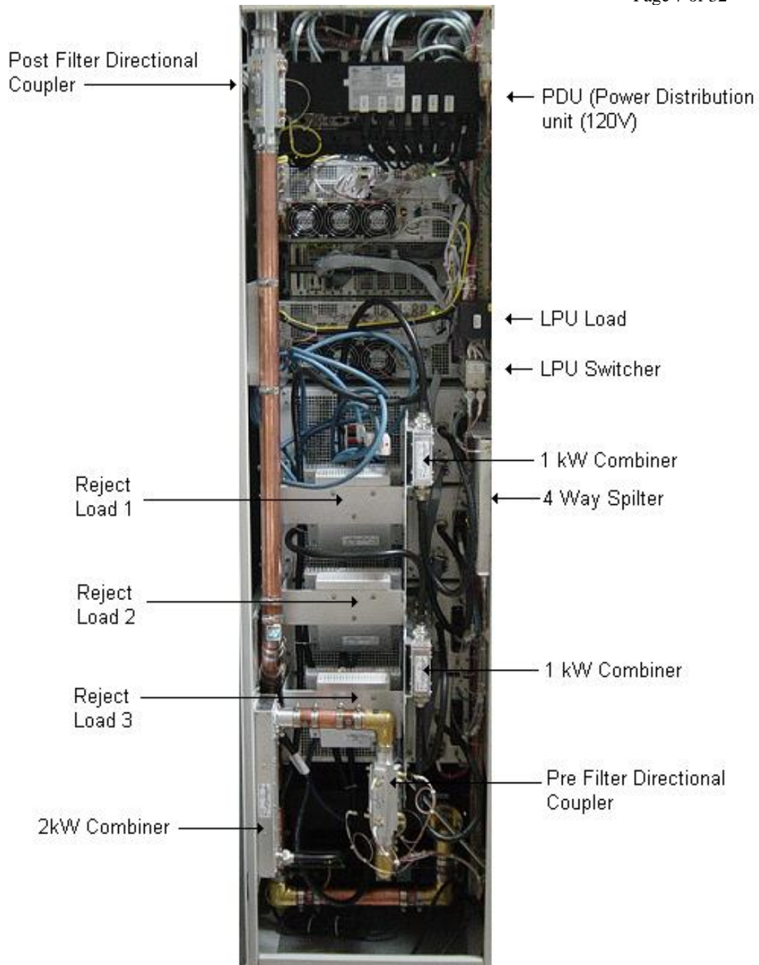
Figure 4, UAX Rear View, Door Removed
