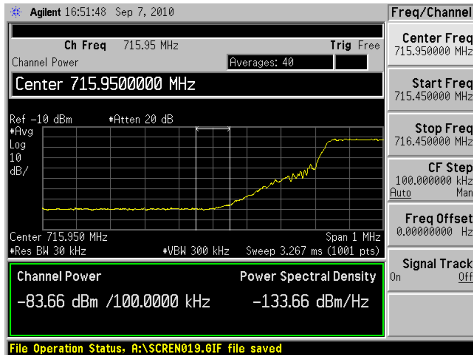
Figure12, Lower Adjacent Channel Power
