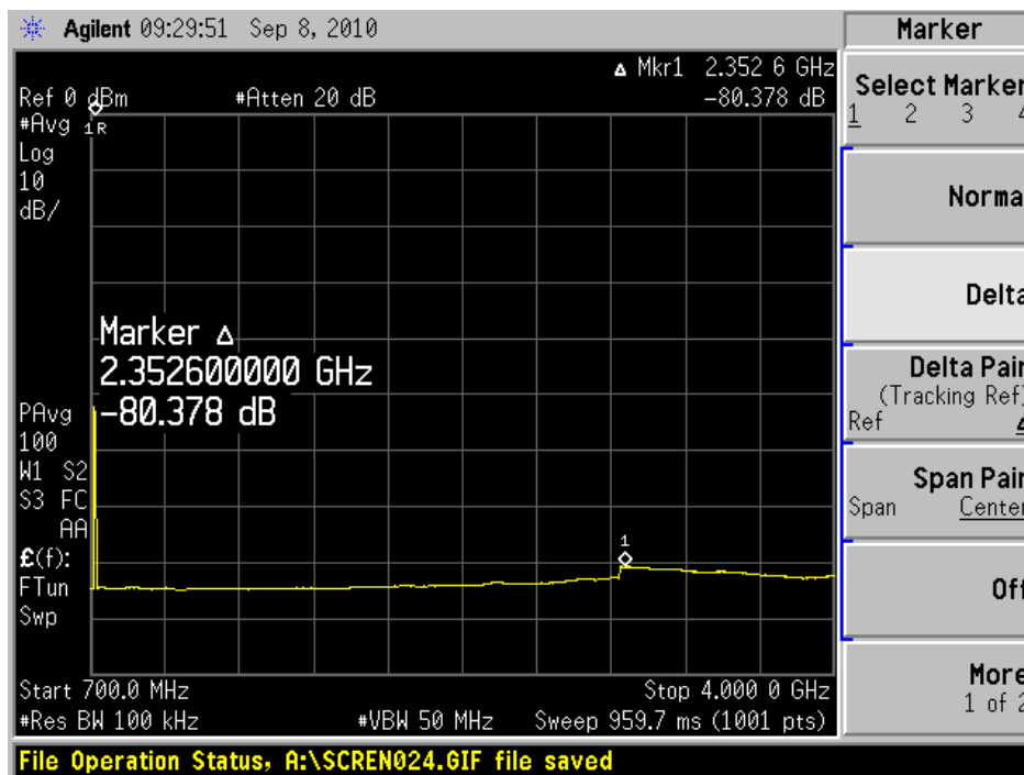
Figure 19, 700 MHz to 4.0 GHz
