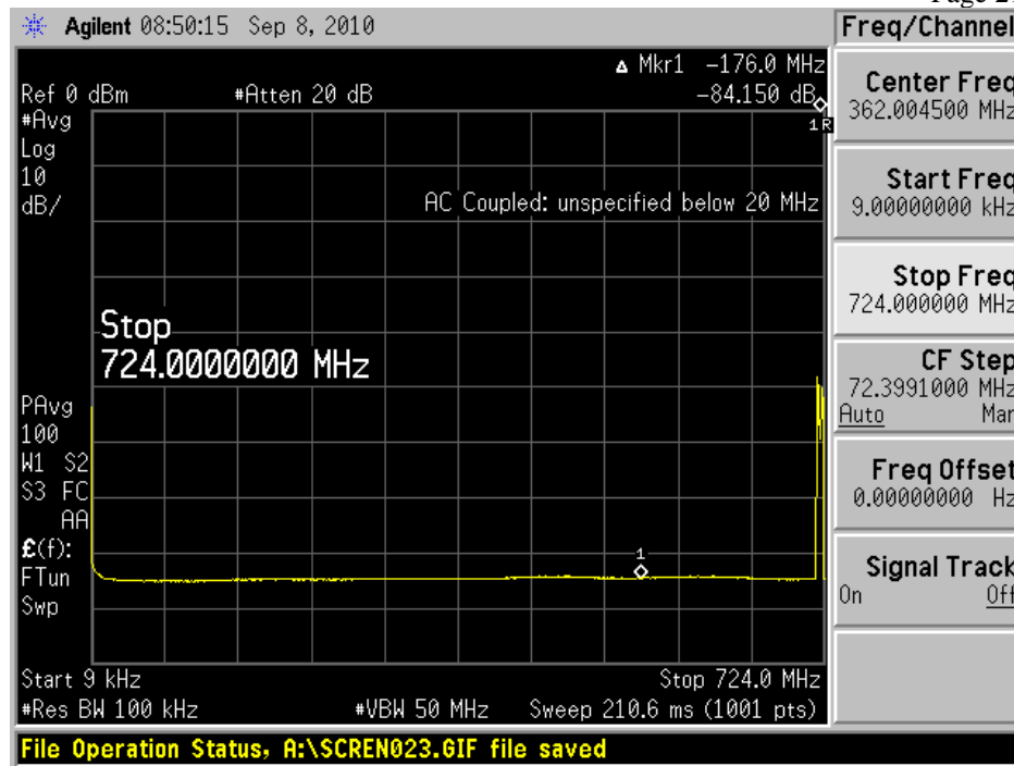
Figure 18, 9 kHz to 724 MHz
