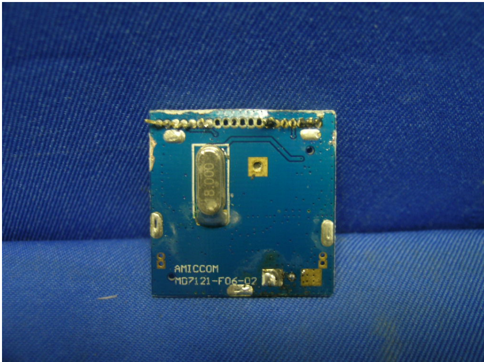
Internal Photo – 14
