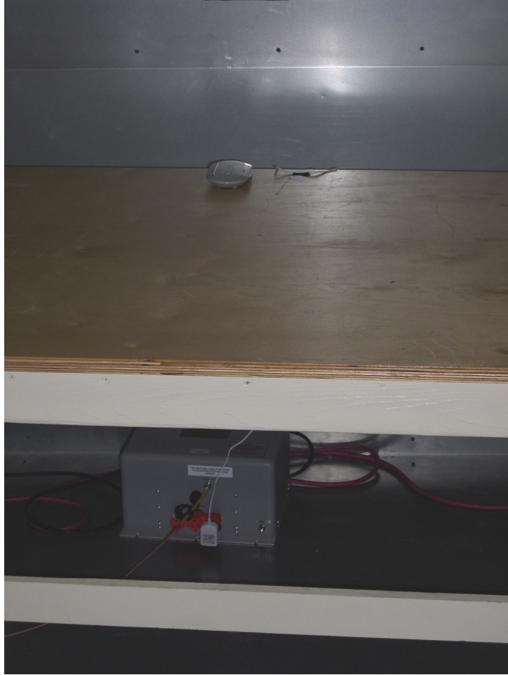
AC Mains Conducted EMI
