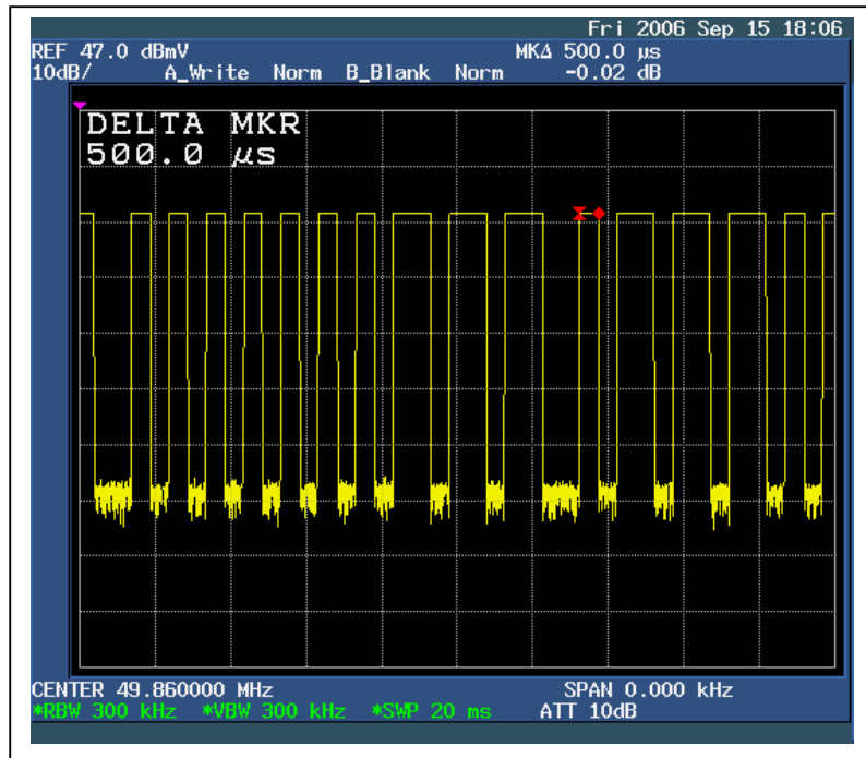
Duty Cycle 3
