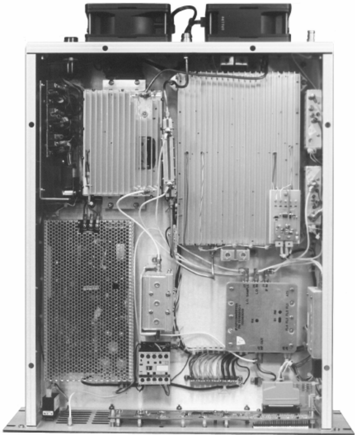
TU20F Exciter Upconverter Internal View
