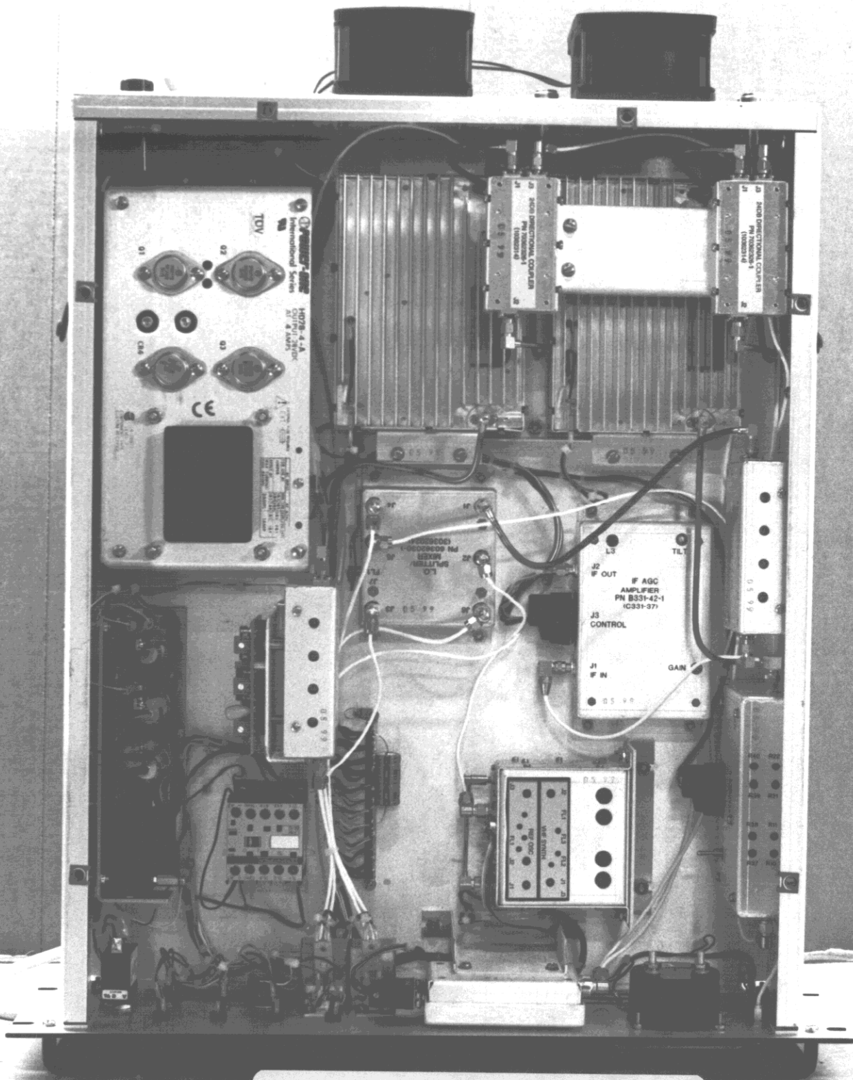
2W VHF EXCITER INTERNAL Photo 2-15C
