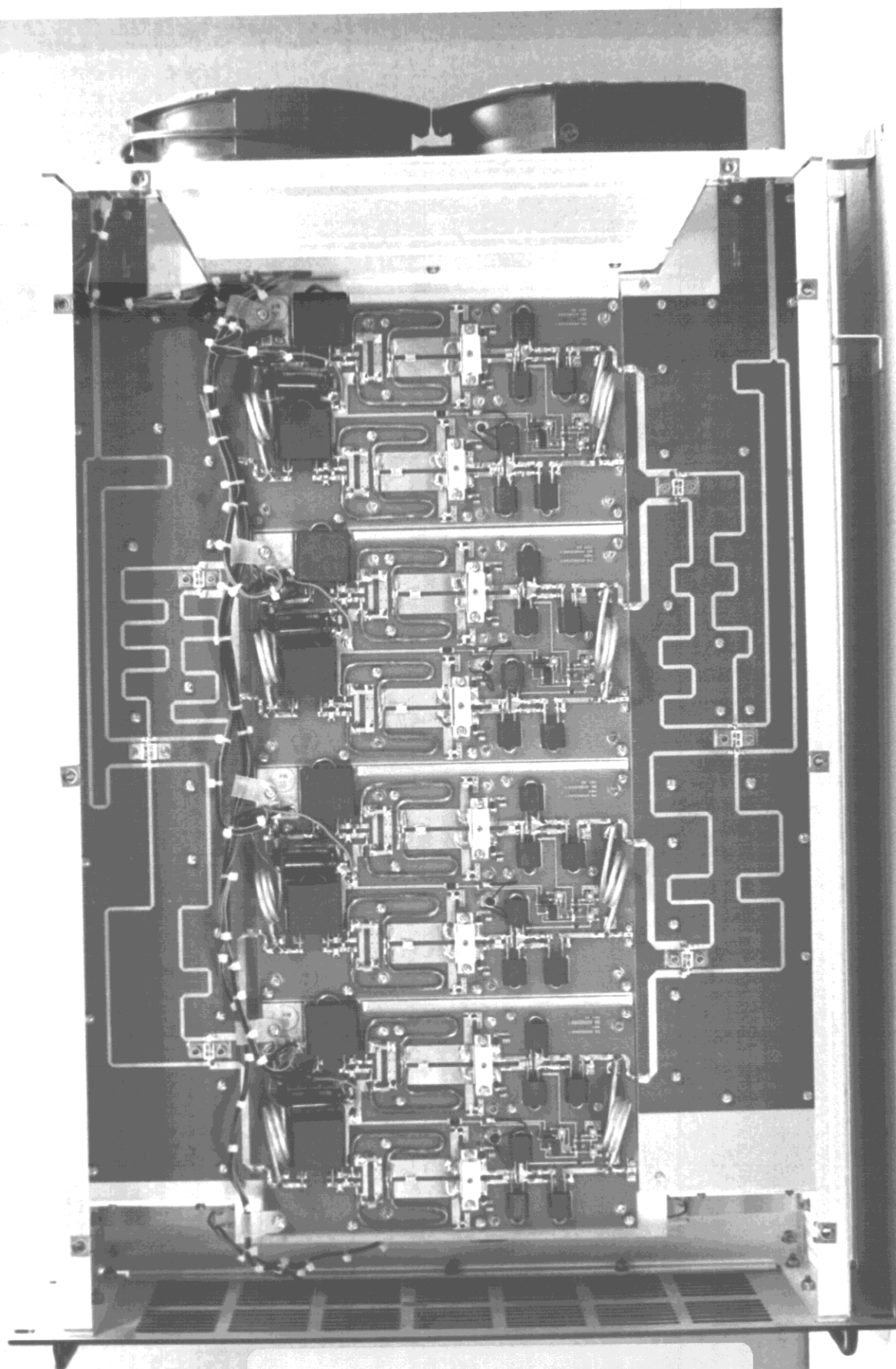
1000W VISUAL FINAL AMPLIFIER INTERNAL Photo 2-15E
