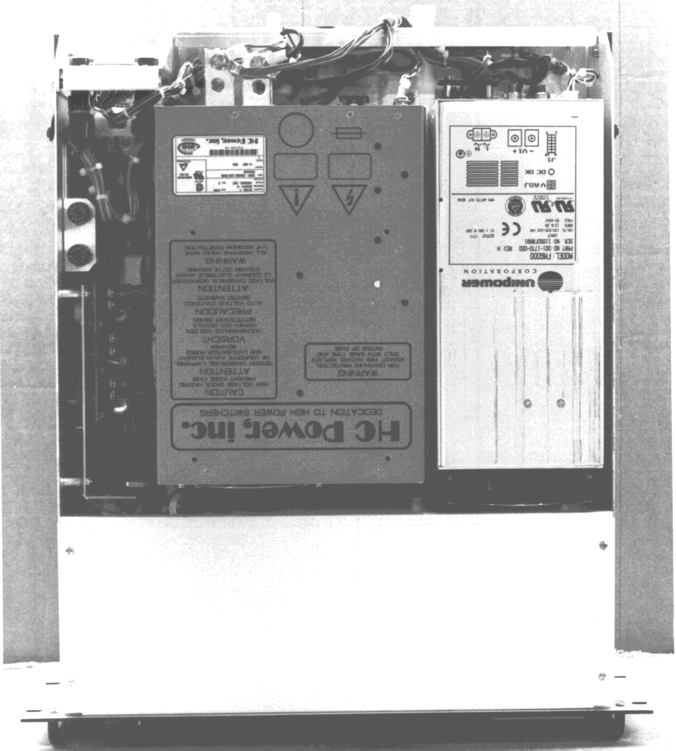
POWER SUPPLY/CONTROL STATUS DRAWER INTERNAL Photo 2-15F
