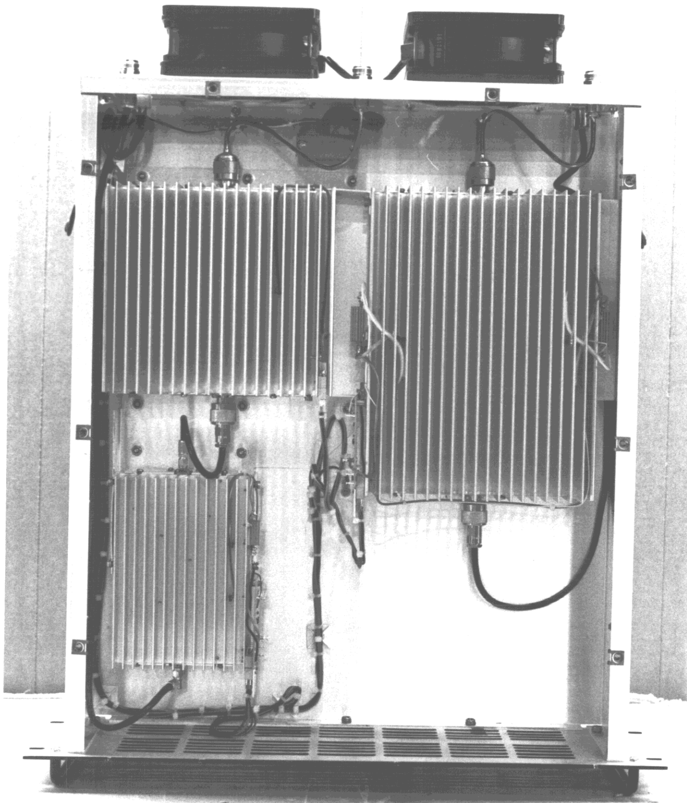
VISUAL IPA/AURAL FINAL INTERNAL Photo 2-15D
