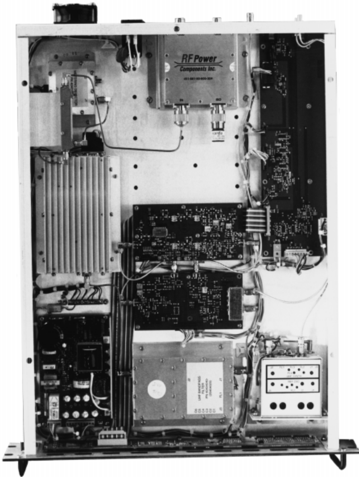
EMEX1 2W UHF Exciter Internal
