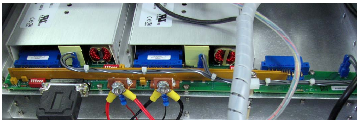
HSD-5000 12Volt Power Supply Backplane
