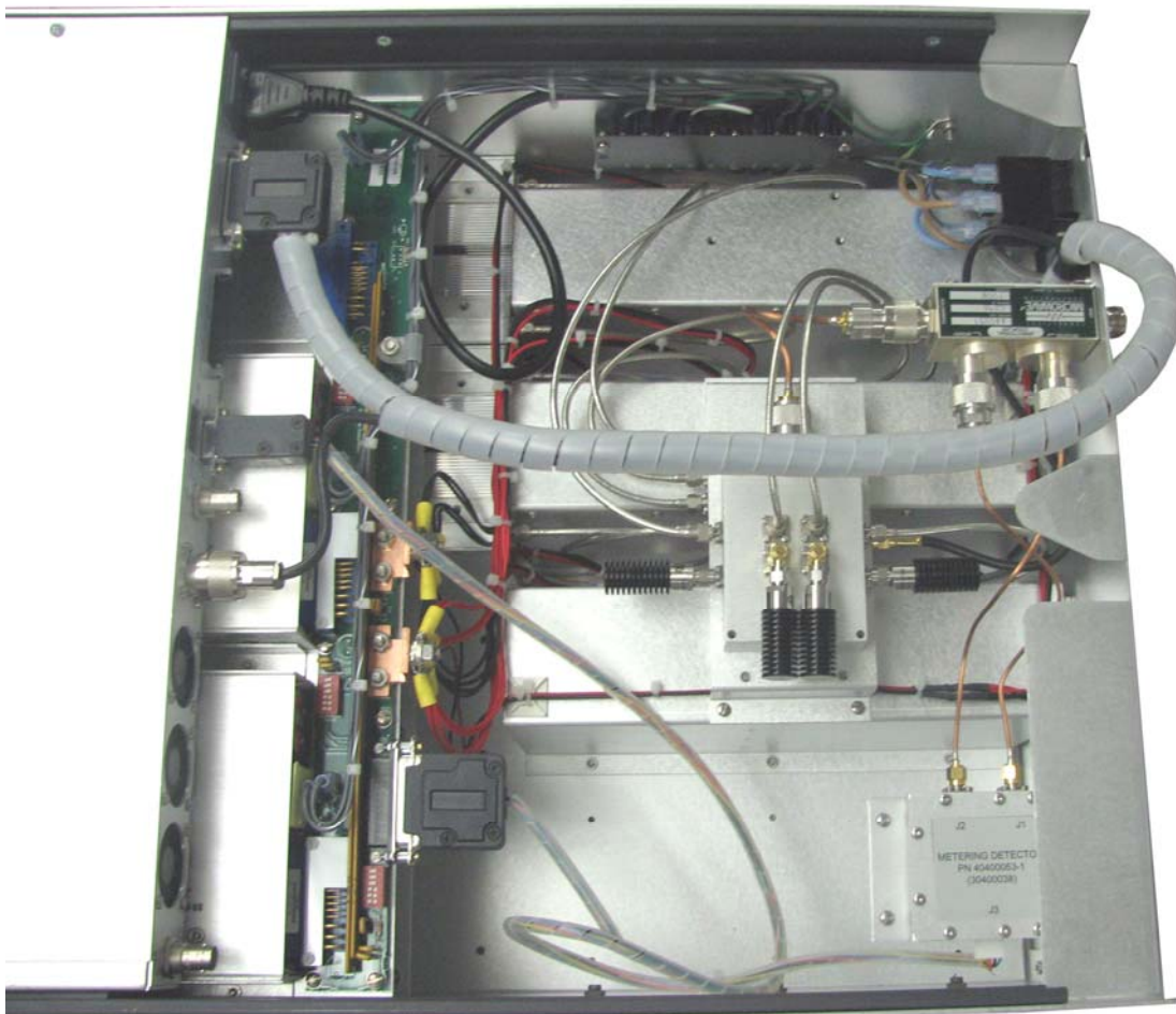
HSD-5000 Main Chassis
