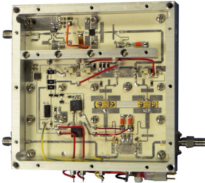
HSD-5000 Up-Converter Output Amplifier
