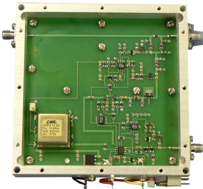
HSD-2500 10 MHz Reference Oscillator
