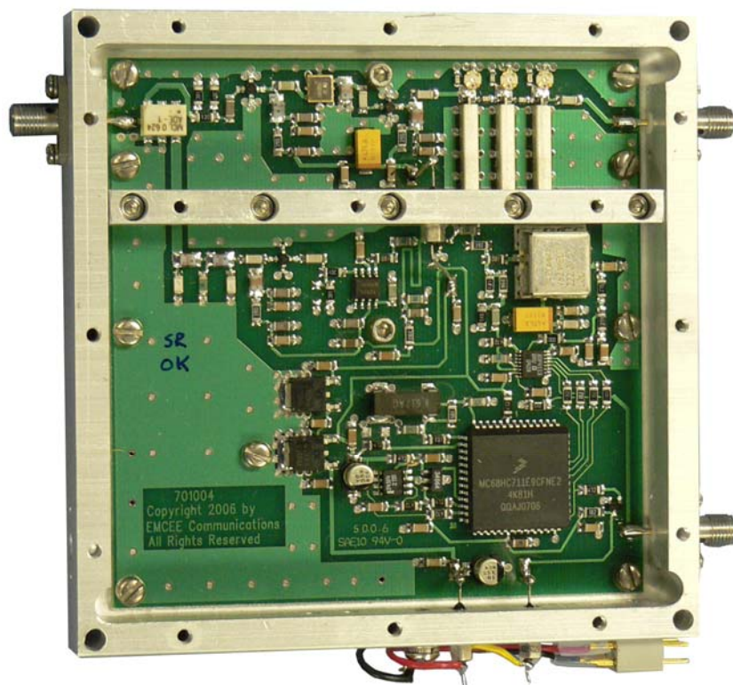
HSD-2500 1 st Converter Module
