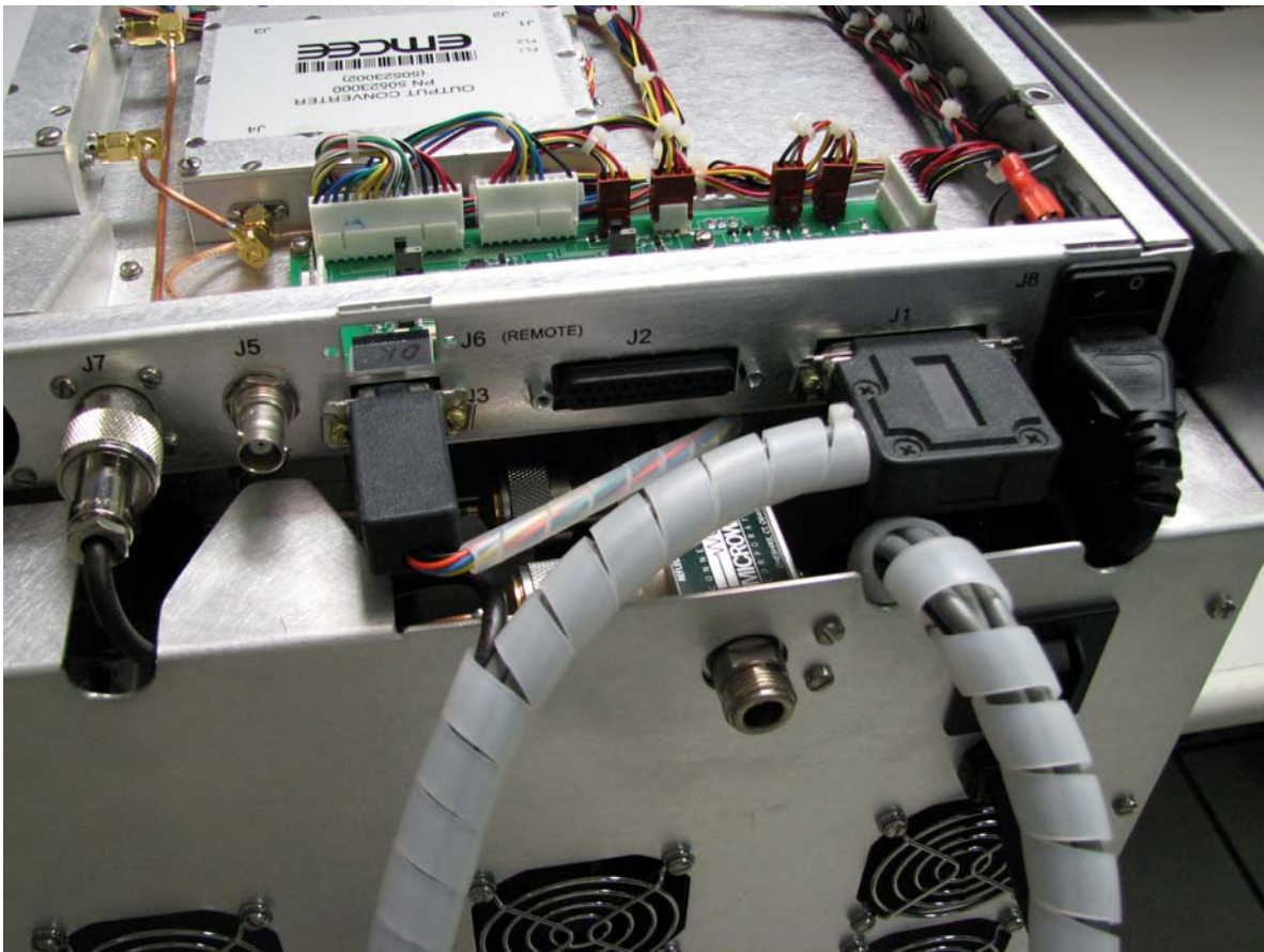
HSD-2500 Chassis Interconnection
