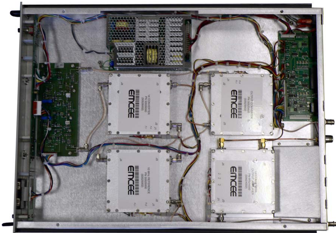
HSD-2500 Up-Converter Drawer
