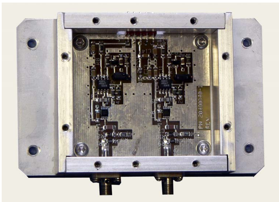
HSD-2500 Metering Detector Module
