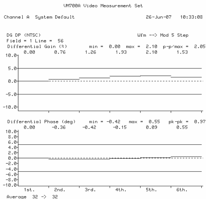
Figure 4-9: Differential Gain & Phase Plot
