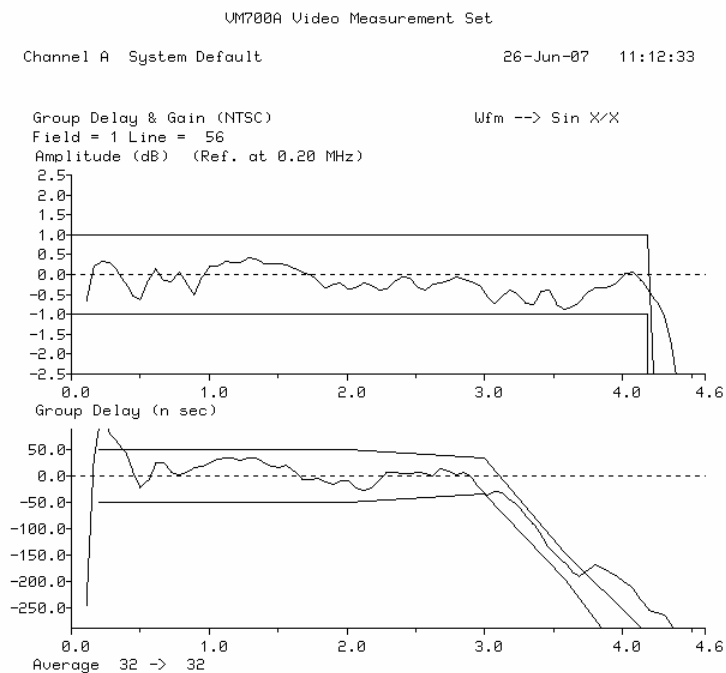
Figure 4-7 Group Delay & Gain Measurement Plot
