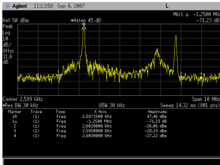
Figure 4-13: Out of Band Attenuation for Analog Operations
