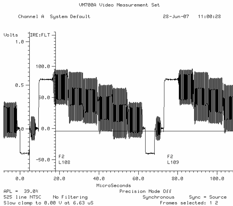
Figure 4-6: Substantially Linear Demodulated Video Waveform Plot
