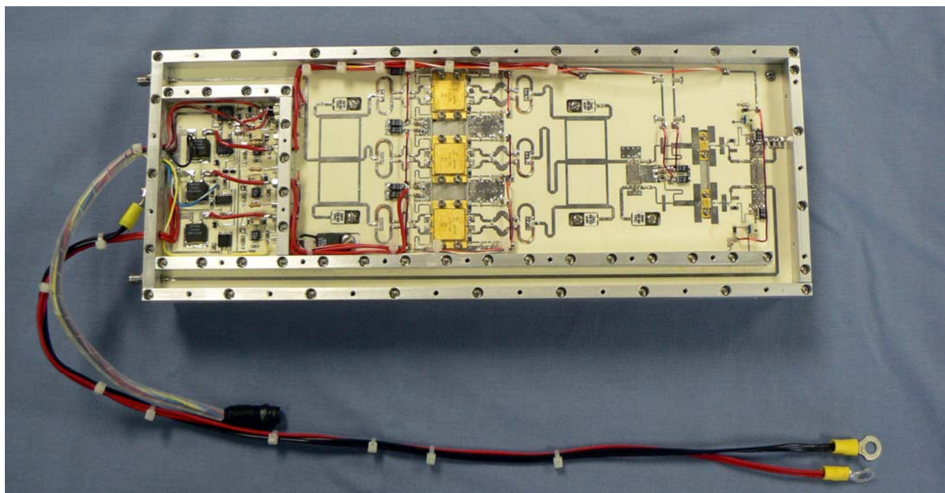
HSD-1250 12.5 Watt Power Amplifier
