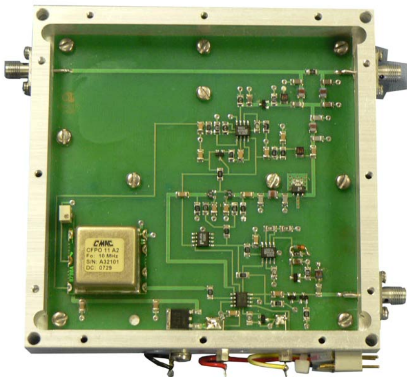
HSD-1250 10 MHz Reference Oscillator
