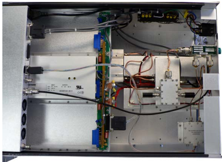
HSD-1250 Main Chassis
