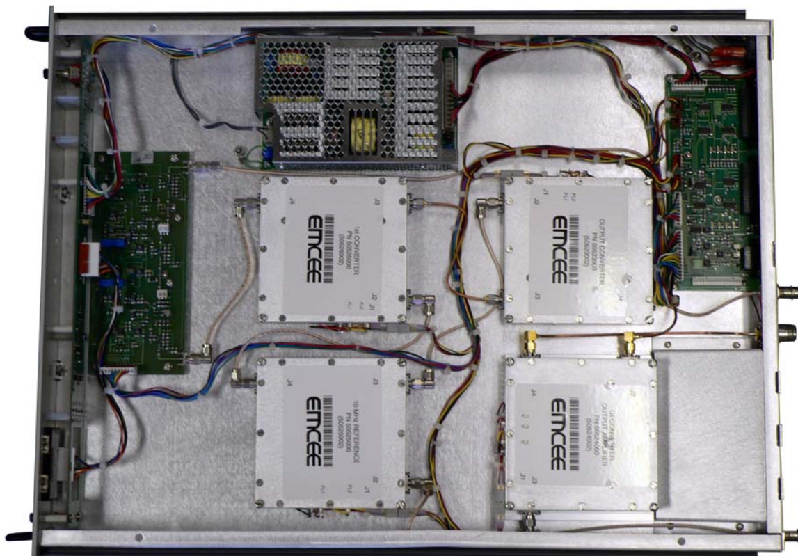
HSD-1250 Up-Converter Drawer
