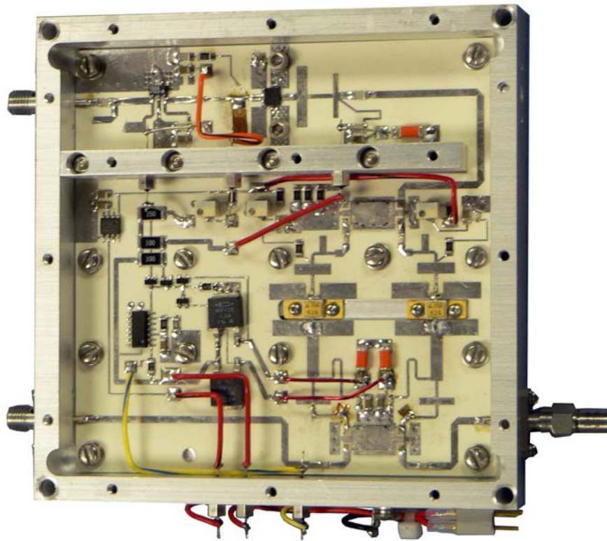
HSD-1250 Up-Converter Output Amplifier
