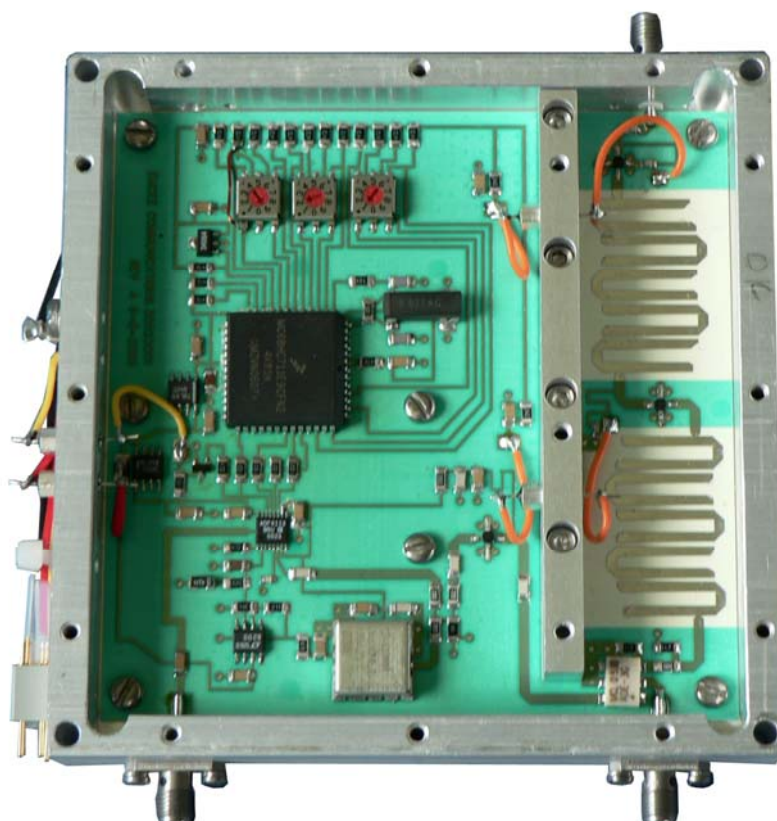
HSD-1250 Output Converter Module
