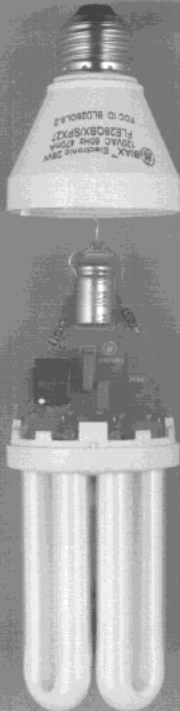
Exhibit F Construction Detail Model # FLE28QBX FCC ID: BLD280LS-2
