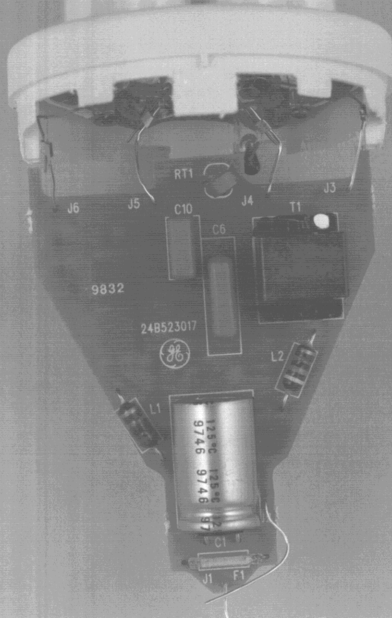
Exhibit G#1A Component Placement Model # FLE24TBX FCC ID: BLD24HLS-1
