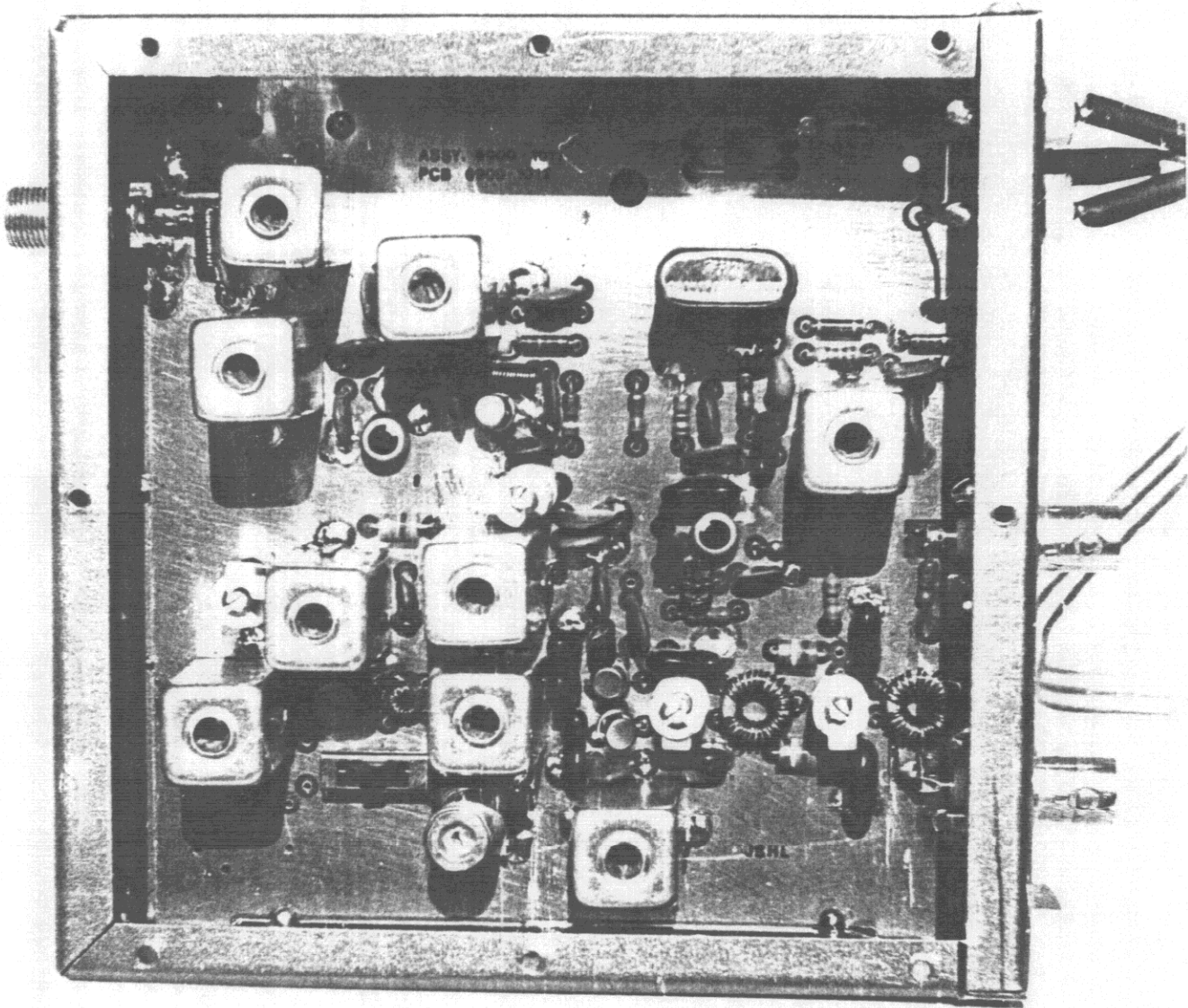
EXHIBIT 9J DETAIL OF INPUT CONVERTOR MODULE WITH COVER REMOVED
