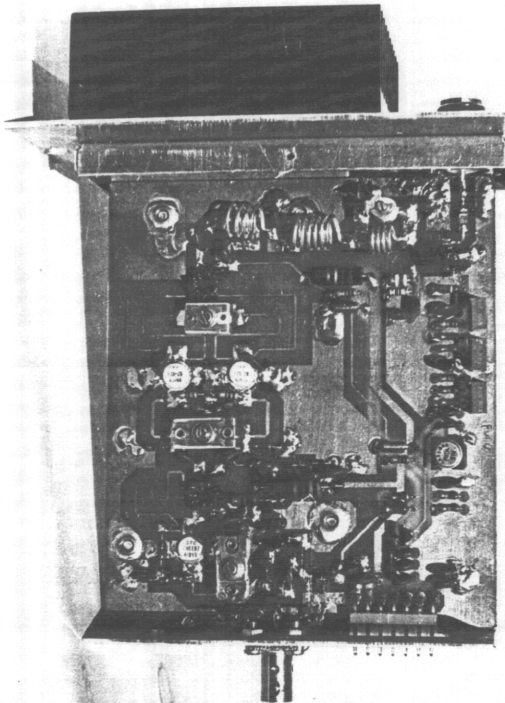
EXHIBIT 9I DETAIL OF POWER AMPLIFIER MODULE WITH COVER REMOVED
