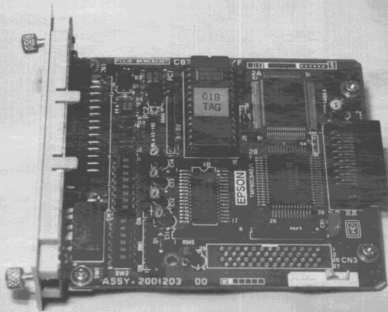
FCC ID BKMFBX1A-1 21) Optional Serial Interface card (SURFACE)
