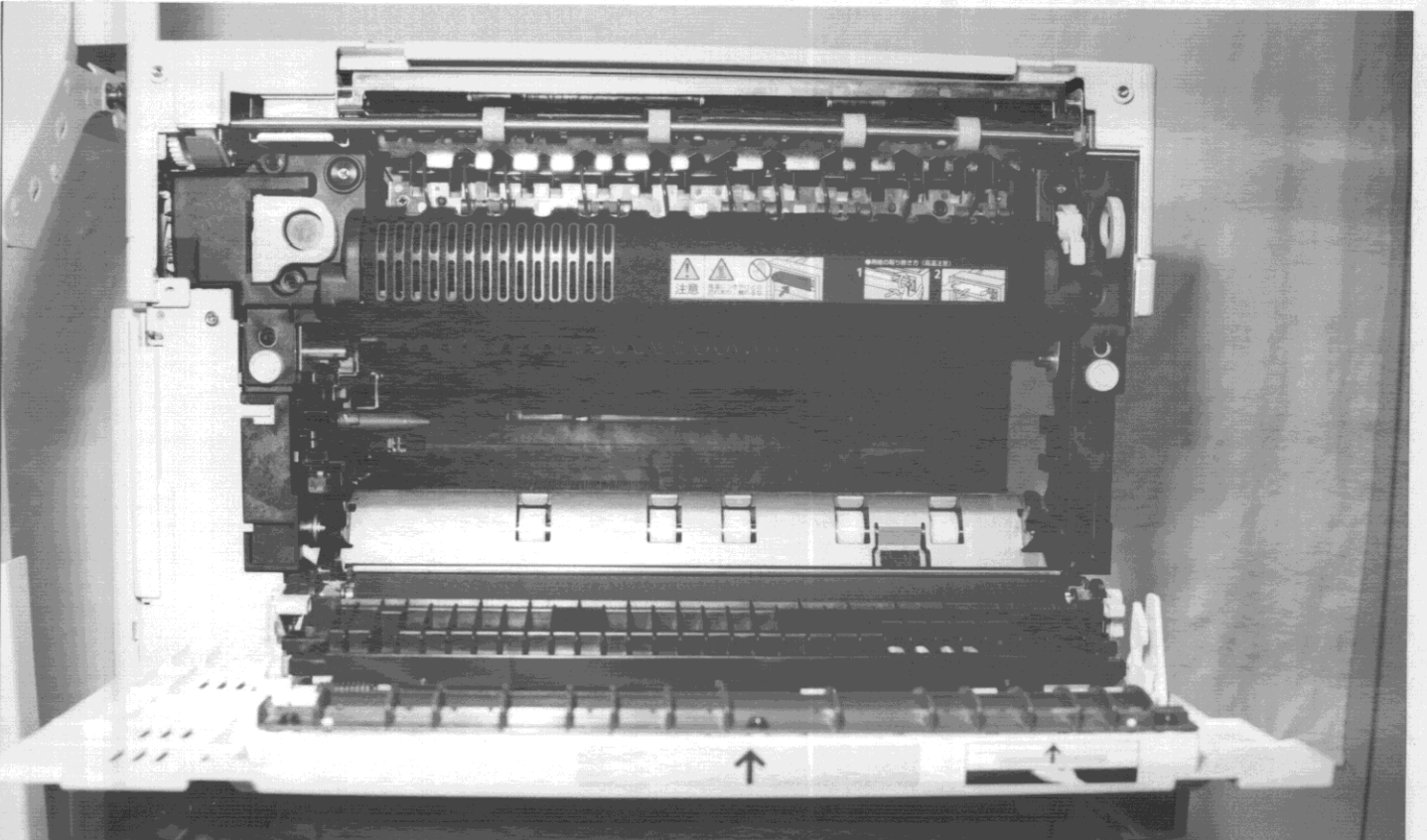
FCC ID BKMFBXYA-1 10) INSIDE VIEW (left side cover open)
