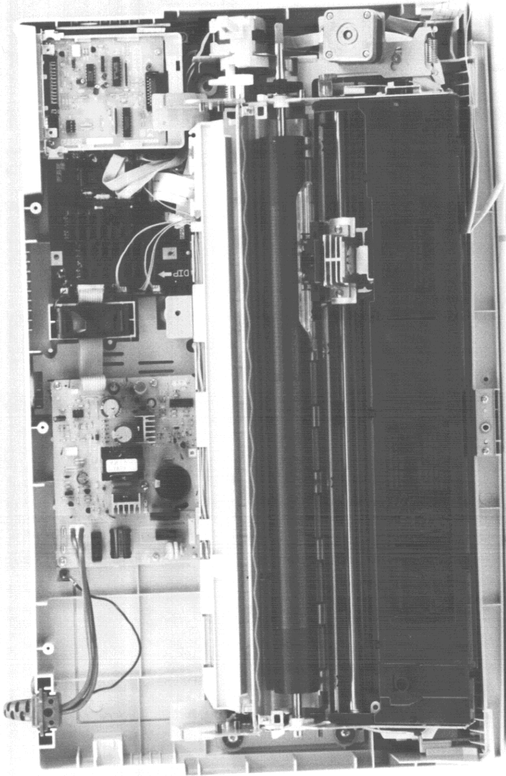
FCC ID : BKMFBP911B 7) Inside view (without steel plate : with options)
