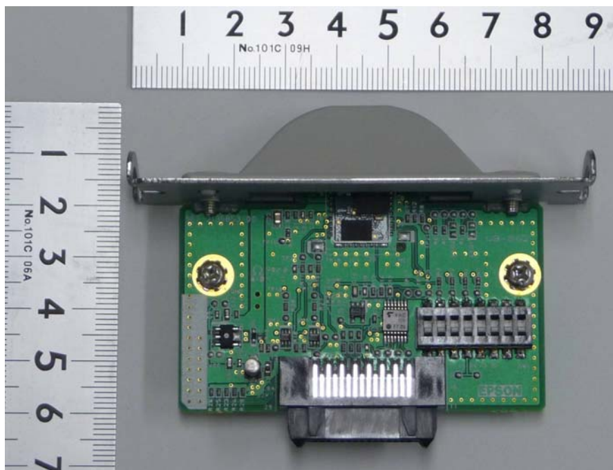
<TOP VIEW>
