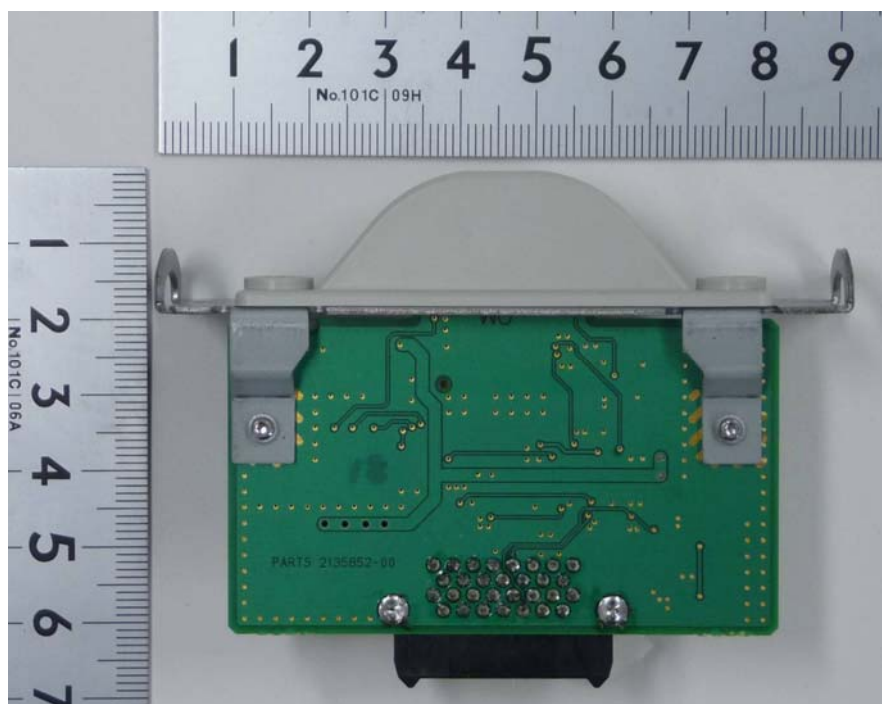
<BOTTOM VIEW>
