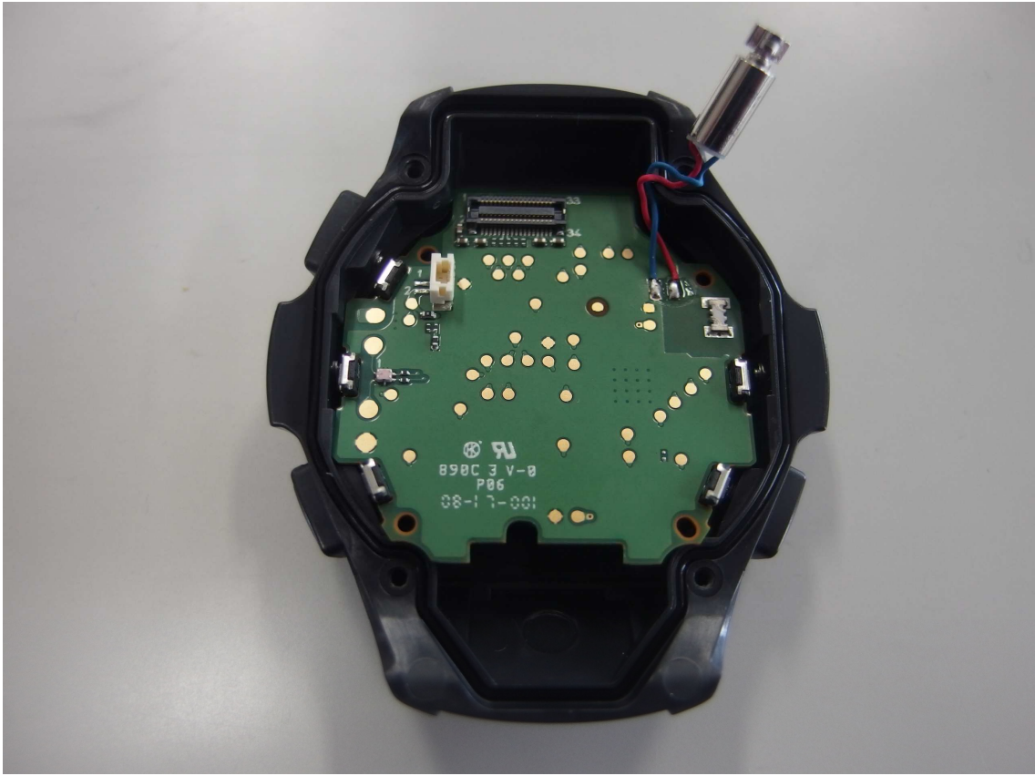
Board layout in case
