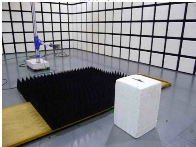
above 1GHz
