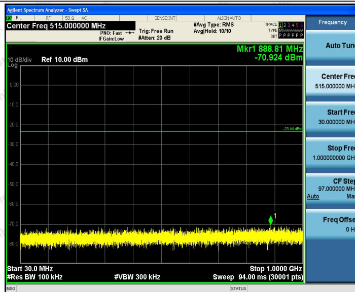
BLE_1M_Ant1_2442_30~1000
