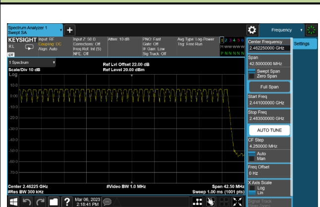
DH5(1Mbps)-2441~2483.5MHz
