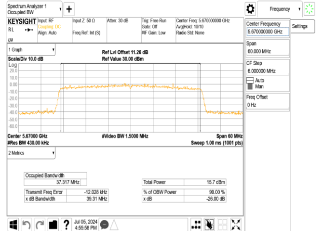
802.11ax_40MHz_Chain0_5670MHz
