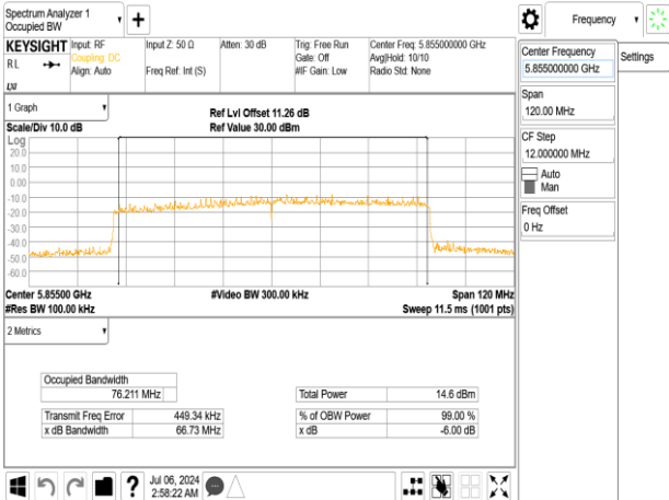
802.11ax_80MHz_Chain0_5855MHz
