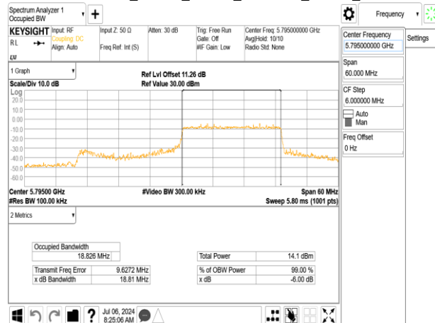
802.11ax_40MHz_Chain0_5795MHz_RU242_62
