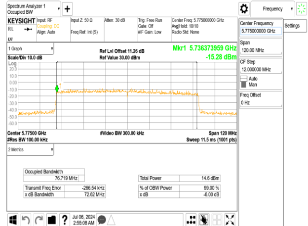
802.11ax_80MHz_Chain0_5775MHz
