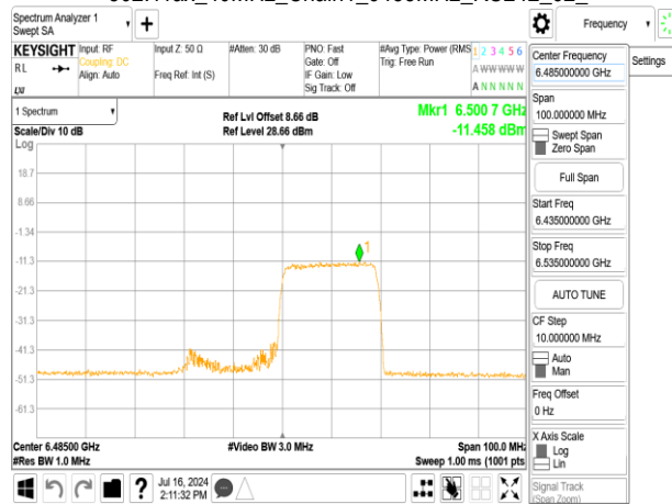
802.11ax_40MHz_Chain1_6485MHz_RU242_62
