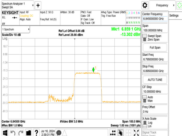
802.11ax_40MHz_Chain0_6845MHz_RU242_62
