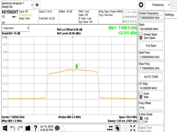
802.11ax_40MHz_Chain0_7085MHz_RU242_62
