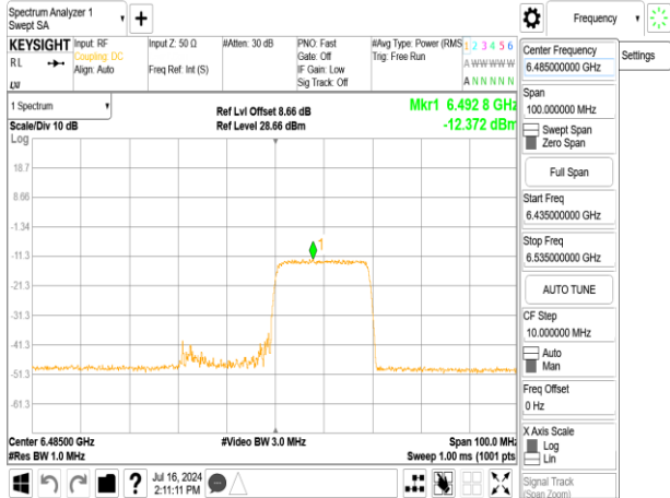
802.11ax_40MHz_Chain0_6485MHz_RU242_62
