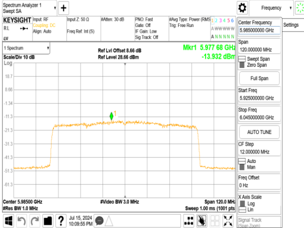
802.11ax_80MHz_Chain0_5985MHz_RU484_65
