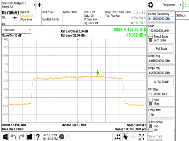
802.11ax_80MHz_Chain0_6145MHz
