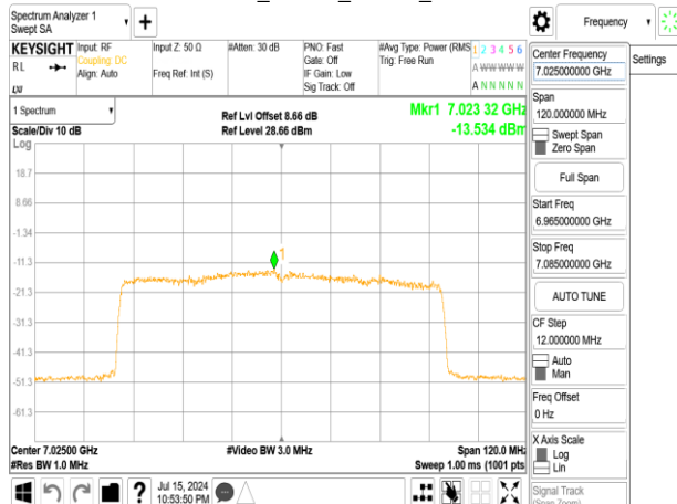
802.11ax_80MHz_Chain0_7025MHz
