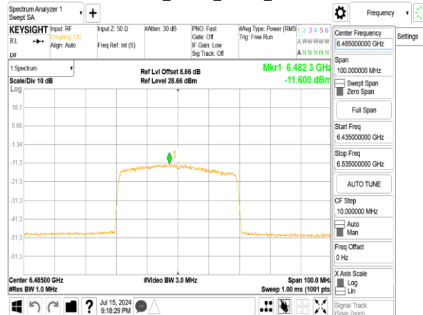
802.11ax_40MHz_Chain1_6485MHz_RU242_62
