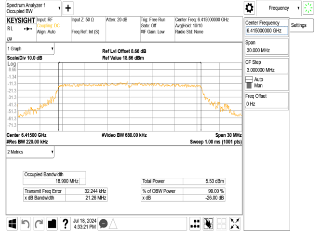
802.11ax_20MHz_Chain0_6415MHz_RU106_54
