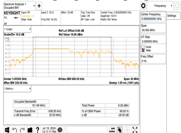
802.11ax_20MHz_Chain0_5955MHz_RU106_53
