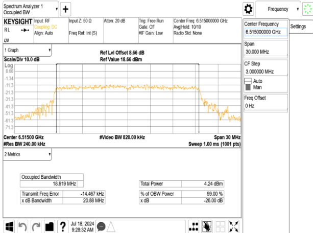
802.11ax_20MHz_Chain0_6515MHz_RU106_54
