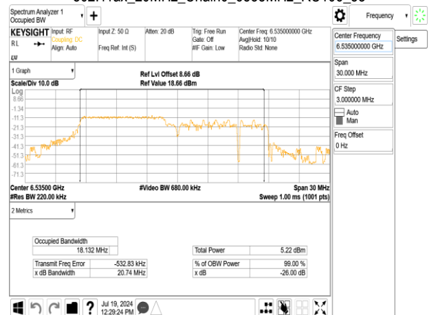
802.11ax_20MHz_Chain0_6535MHz_RU106_53
