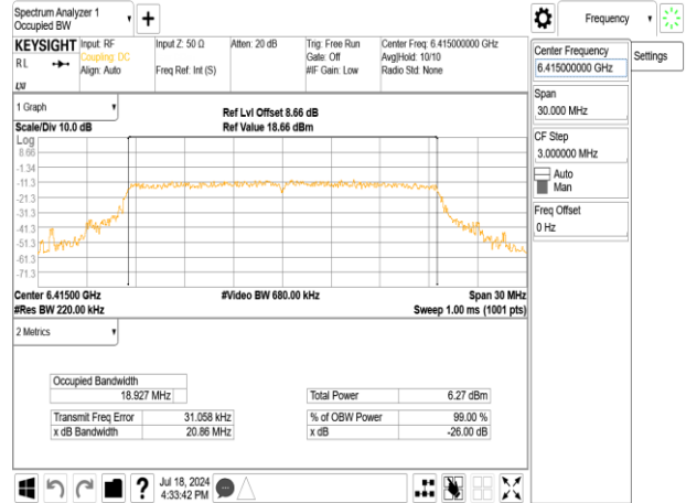
802.11ax_20MHz_Chain1_6415MHz_RU106_54
