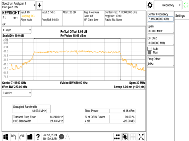
802.11ax_20MHz_Chain0_7115MHz_RU106_54
