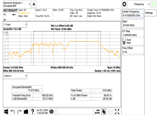
802.11ax_20MHz_Chain0_6415MHz_RU26_8
