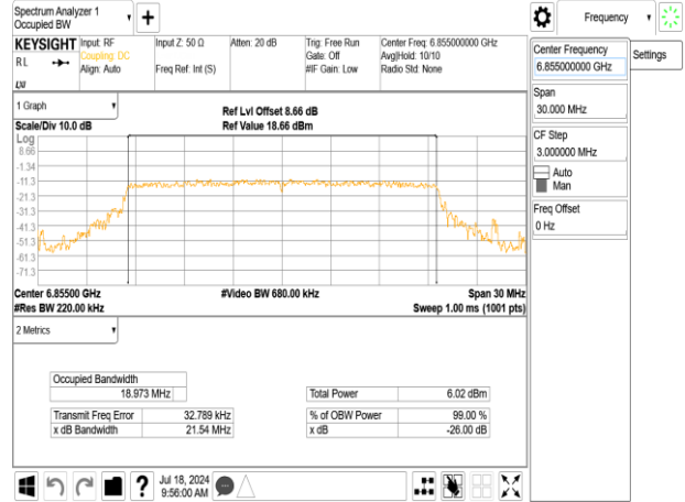
802.11ax_20MHz_Chain0_6855MHz_RU106_54
