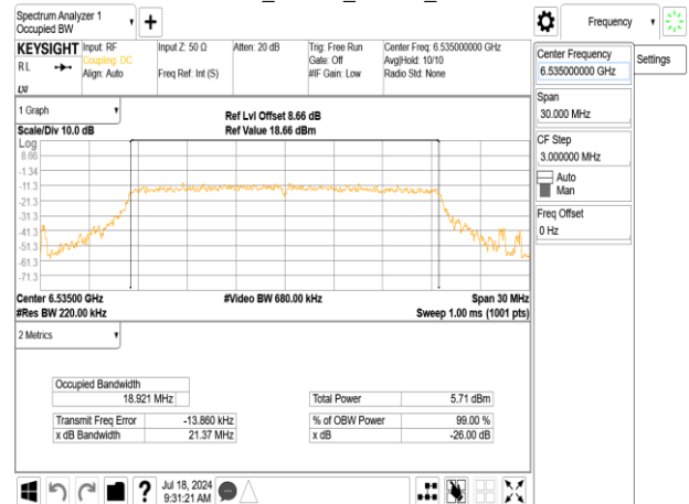
802.11ax_20MHz_Chain0_6535MHz_RU106_53
