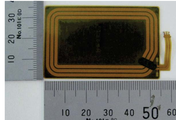
ANT/NFC-RED
