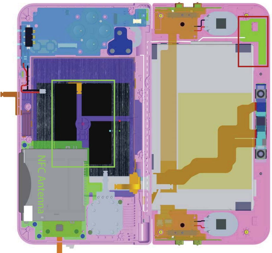
Wi-Fi Antenna
