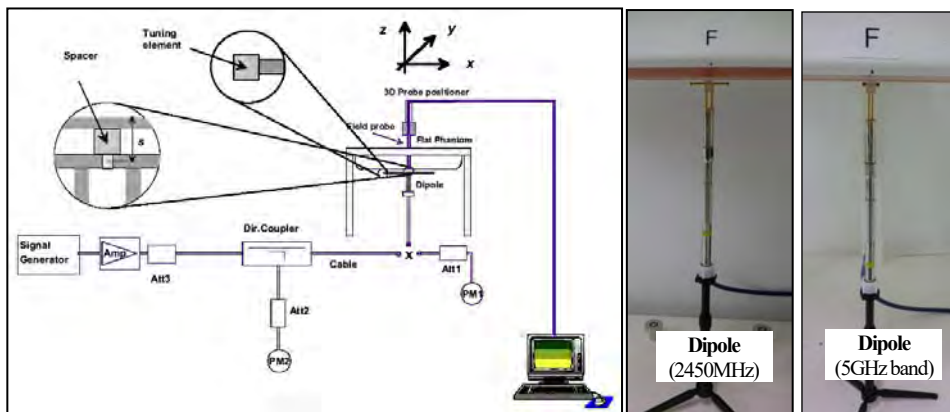
Test setup for the system performance check
