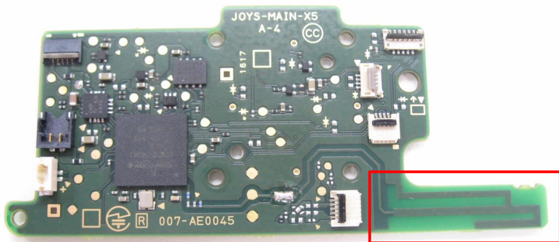
Bluetooth Antenna
