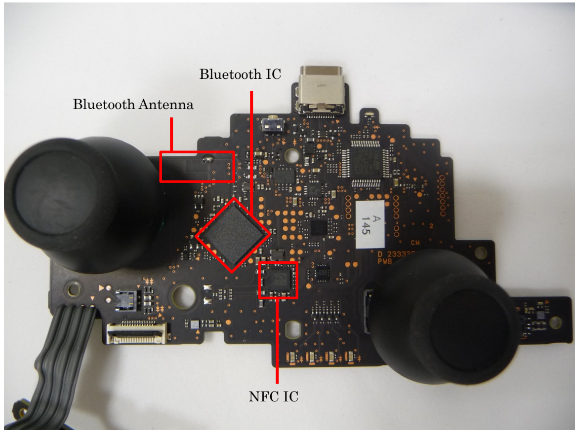
Wireless module PCB (Back):
