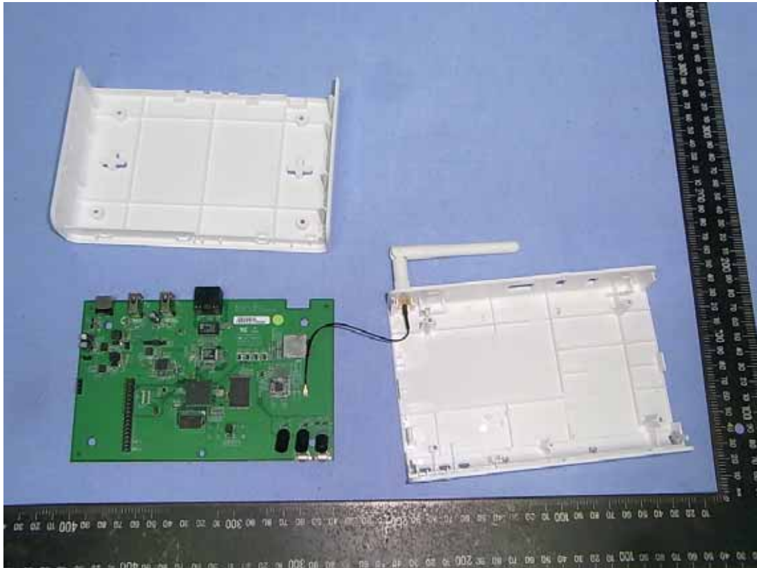
Internal View (Removed Covers)
