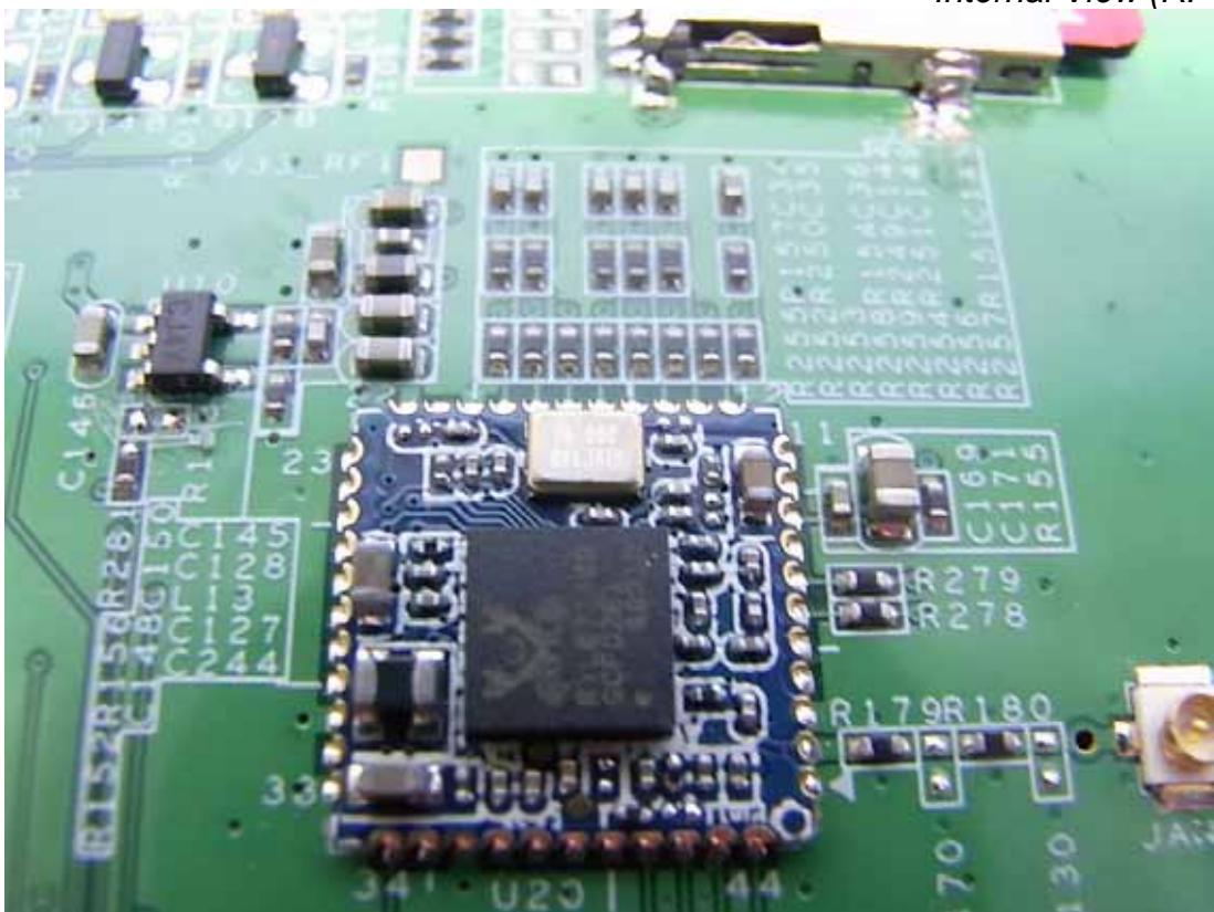
Figure 13 Internal View (RF Module)
