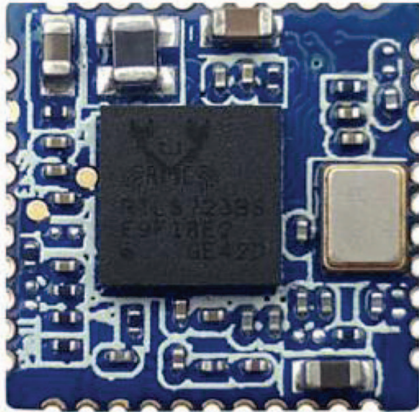
Figure 14 Internal View (RF Module, Front View)
