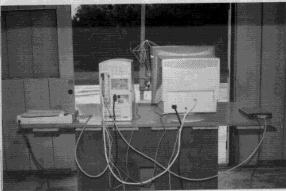
Back View of Radiated Measurement
