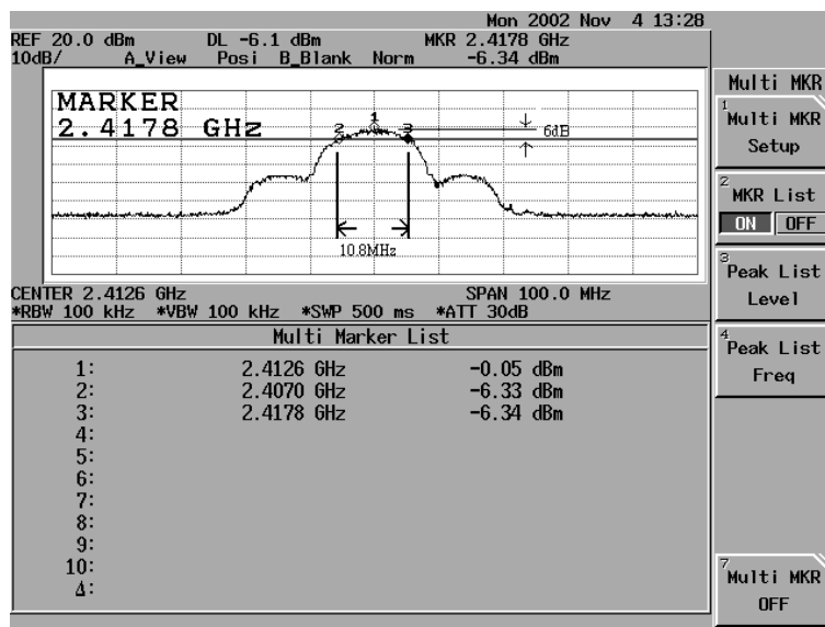
Figure Channel 1: 11Mbps
