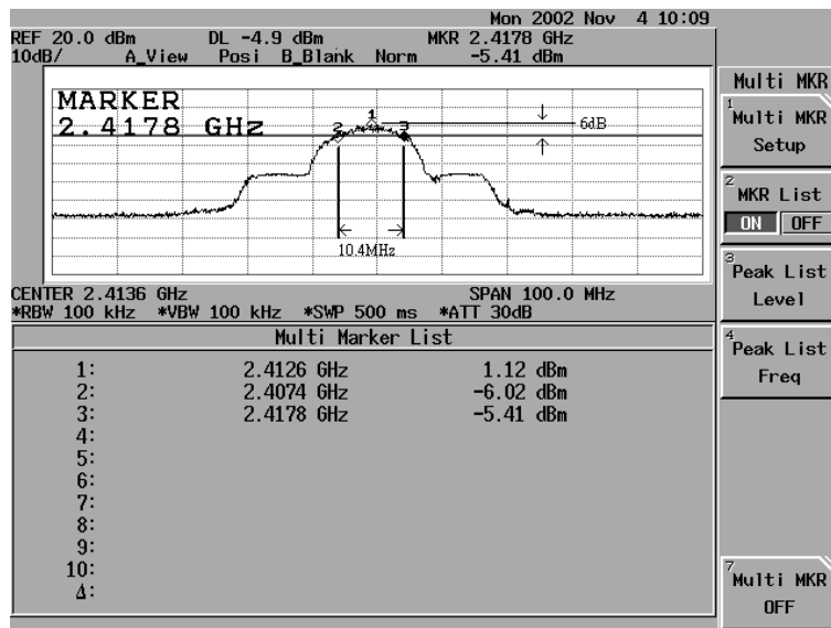
Figure Channel 1: 11Mbps
