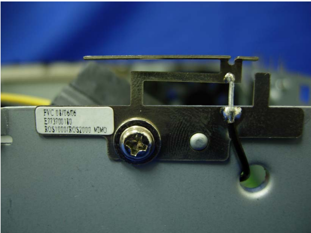
(34) EUT Photo (5GHz-Main)
