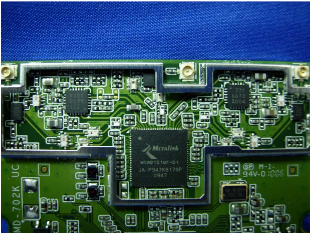
(20) EUT Photo (2.4Hz WLAN Card)
