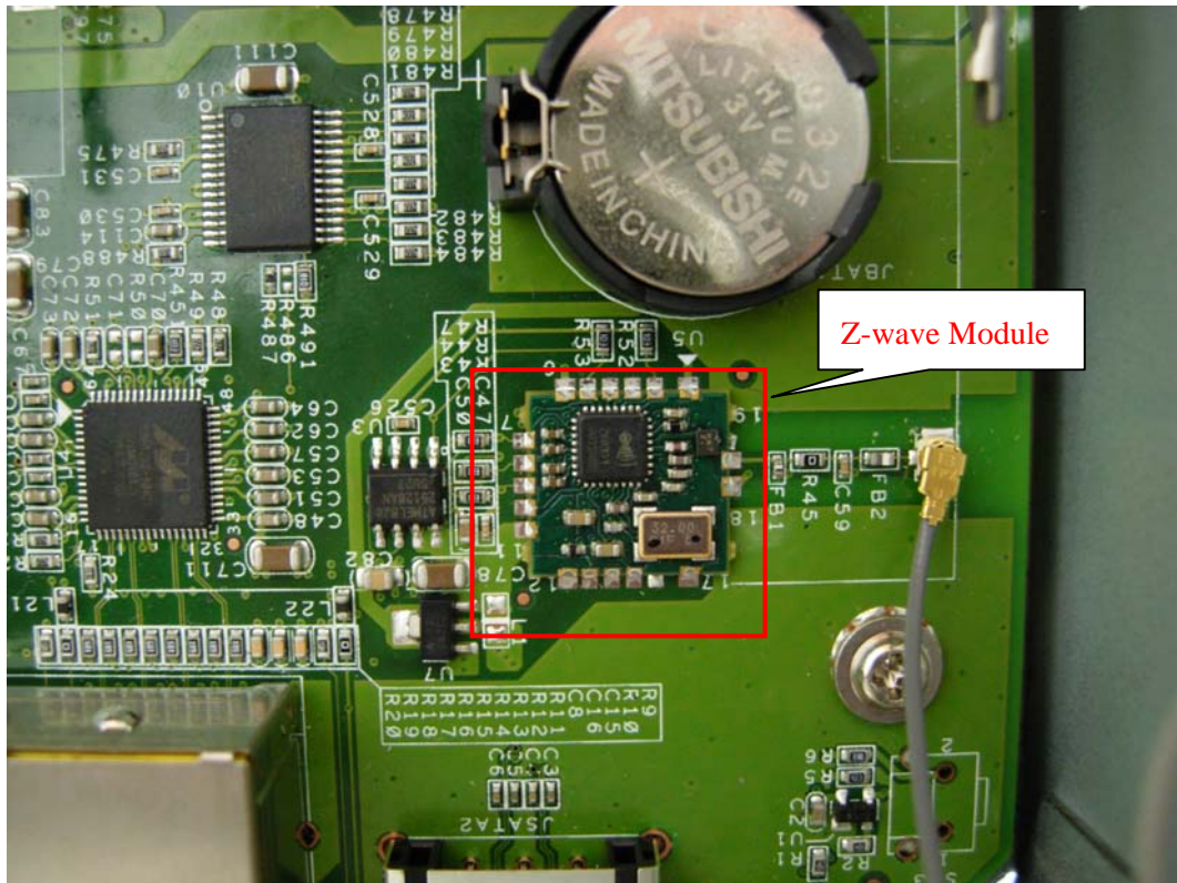
(37) EUT Photo (Z-wave Module)
