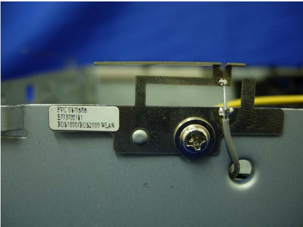
(24) EUT Photo (2.4GHz-Main)
