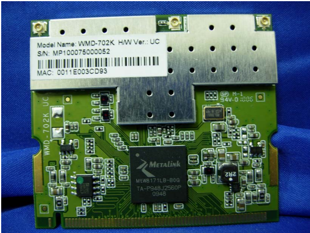
(27) EUT Photo (5GHz-WLAN Card)
