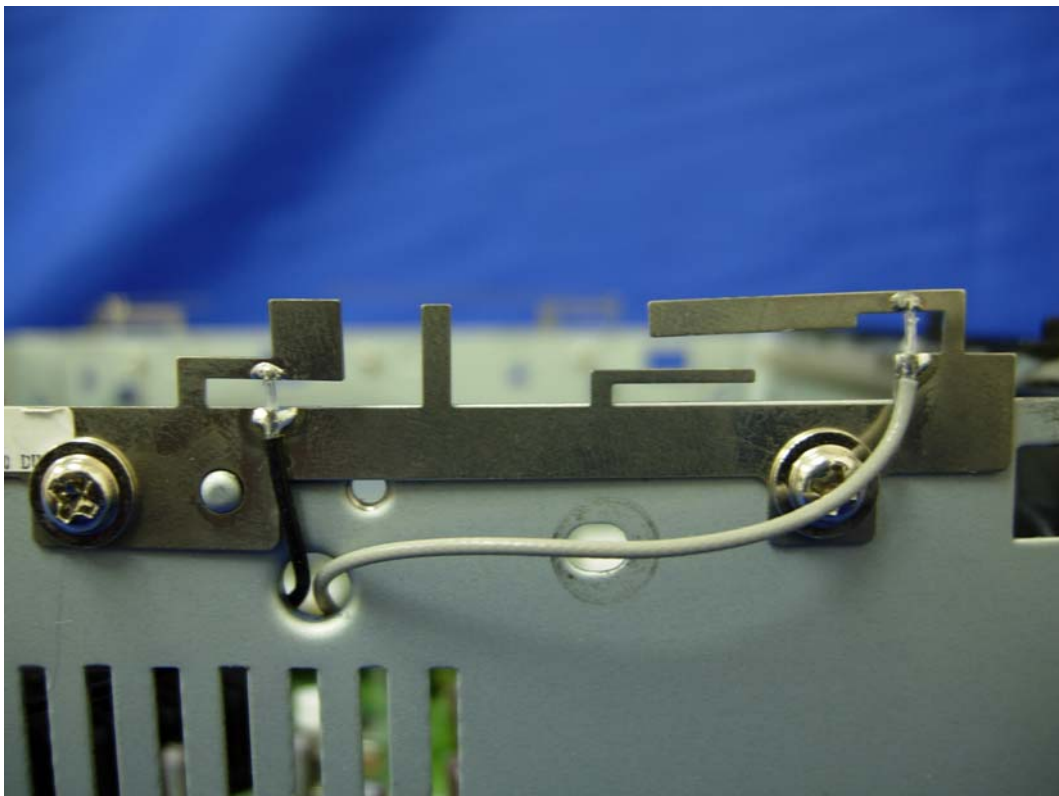
(36) EUT Photo (5GHz-MIMO-black)
