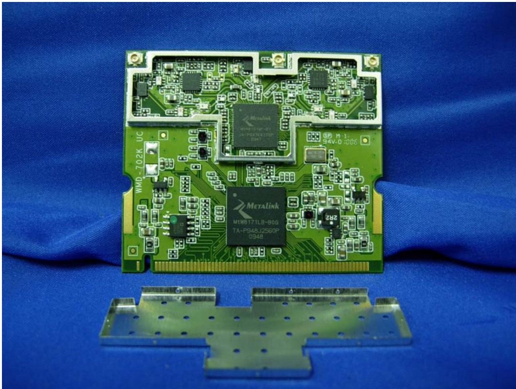
(19) EUT Photo (2.4Hz WLAN Card)
