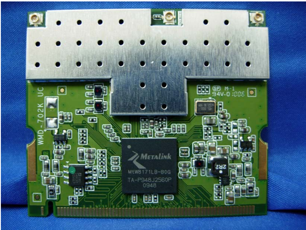
(18) EUT Photo (2.4Hz WLAN Card)
