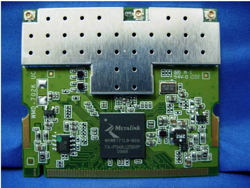
(28) EUT Photo (5GHz-WLAN Card)
