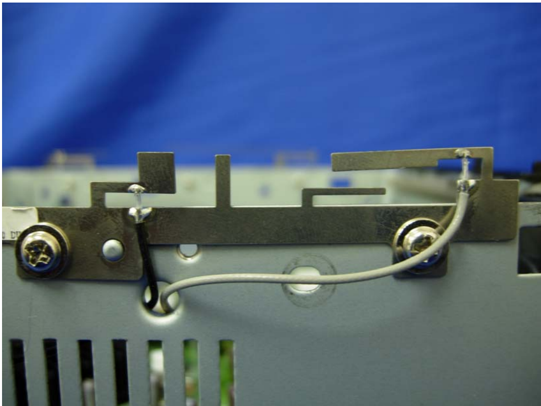
(26) EUT Photo (2.4GHz-MIMO-gray)
