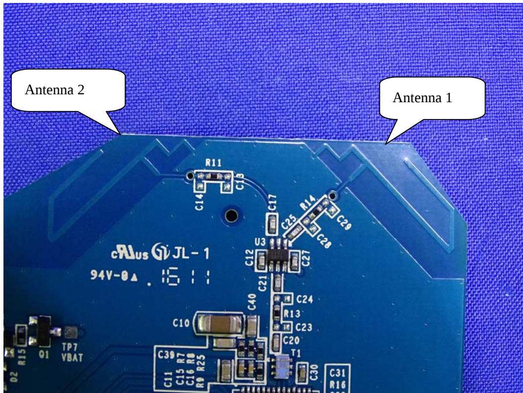
(20) EUT Photo-Antenna
