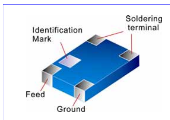
Fig 1. Outline of 2.4GHz Antenna – RFANT3216090A0T
