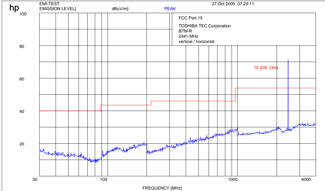
Plot : 0.03 - 4 GHz vertical/horizontal (middle channel)
