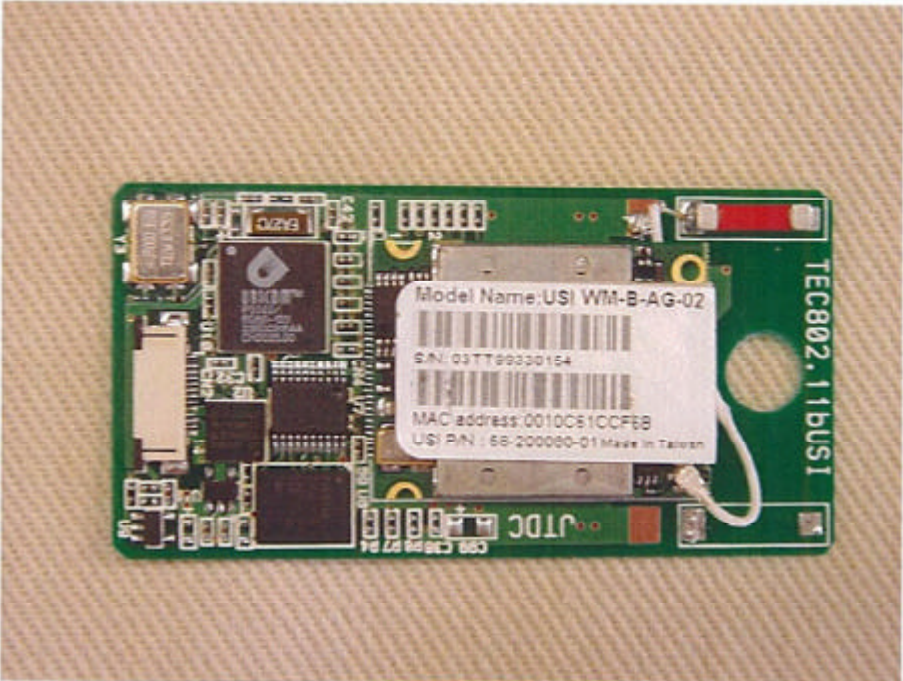
Photo 5 : PCB View : Components Side
