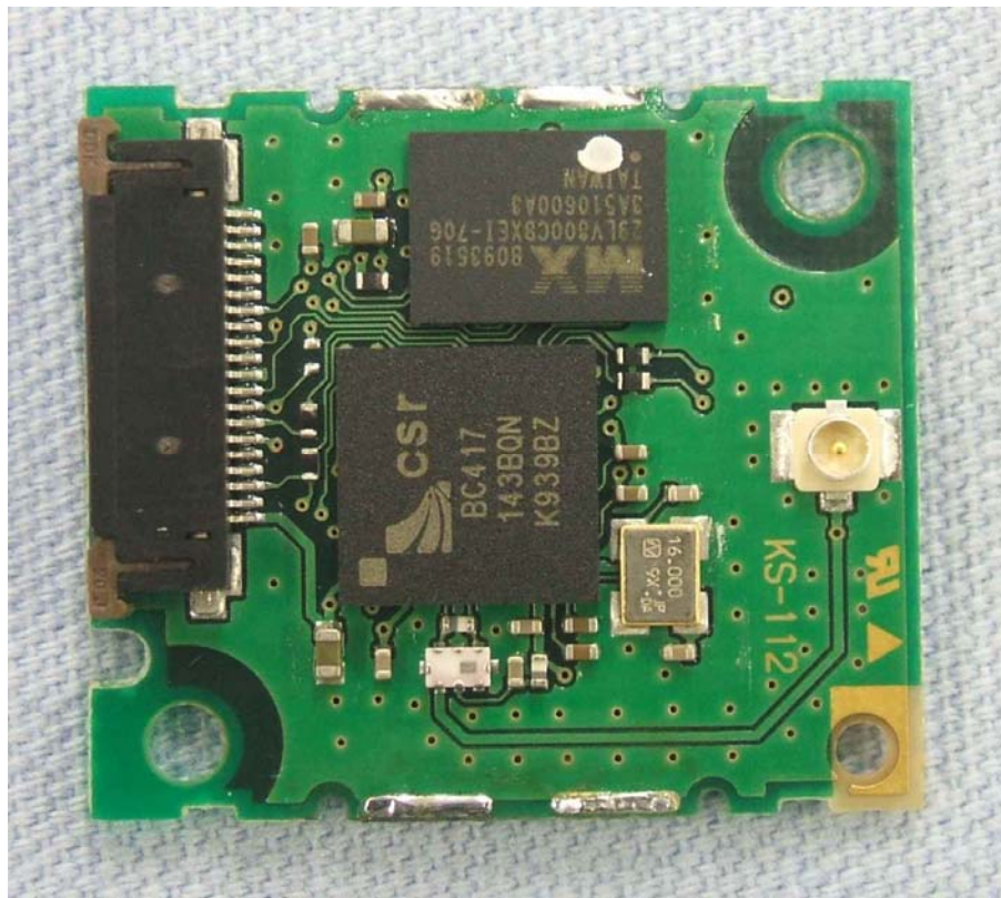
Top – without shield
