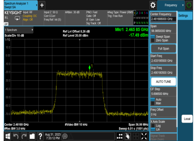
802.11ax_40MHz_Chain1_2452MHz_RU242_62
