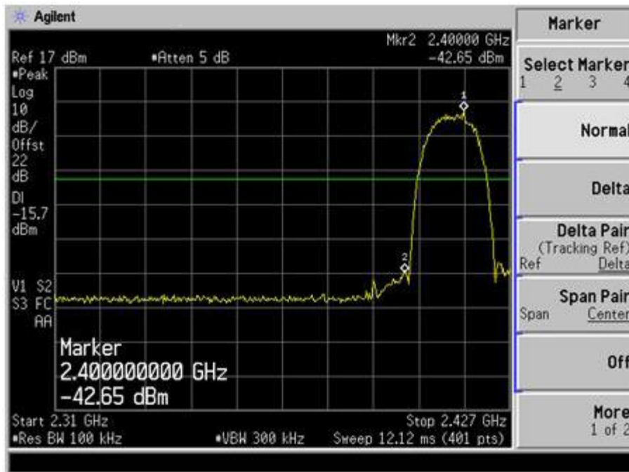
Plot 75 – Lower Band Edge at 2.400GHz @ CCK 5.5Mbps
