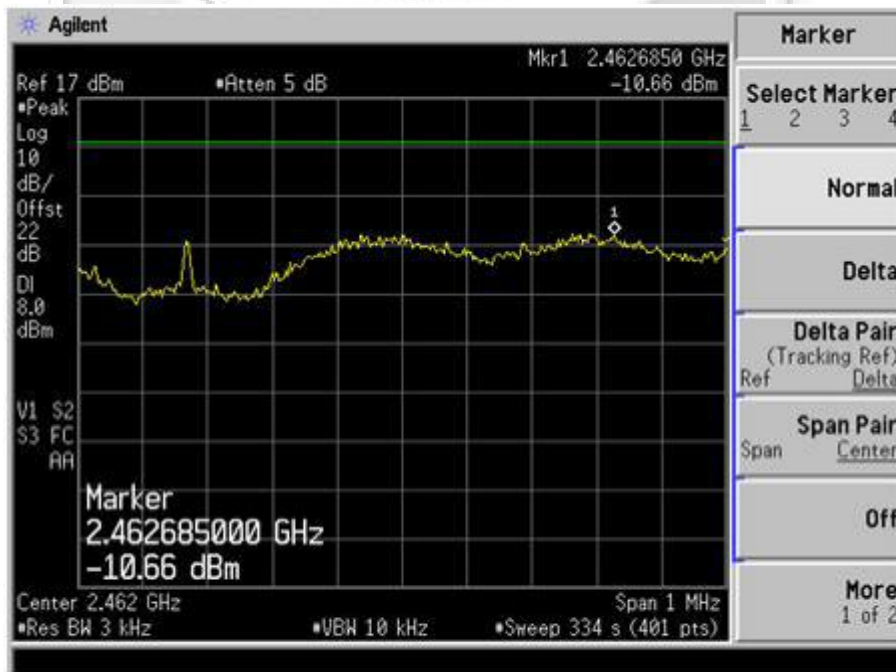
Plot 118 – Channel 11 @ 64QAM 54Mbps
