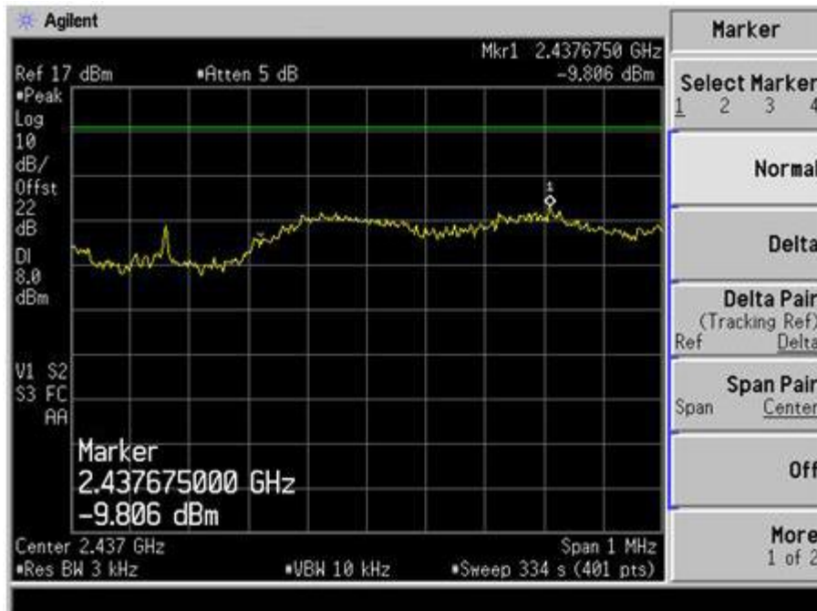
Plot 113 – Channel 6 @ 16QAM 36Mbps
