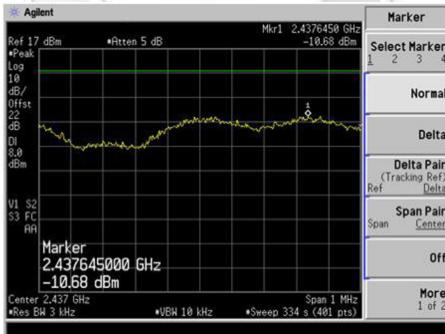
Plot 114 – Channel 6 @ 64QAM 54Mbps
