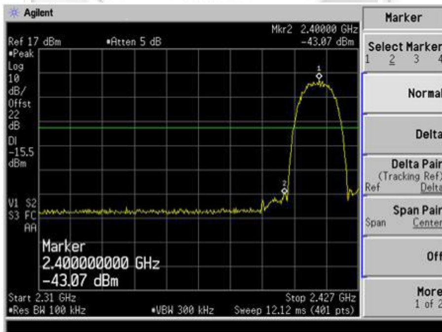
Plot 76 – Lower Band Edge at 2.400GHz @ CCK 11Mbps
