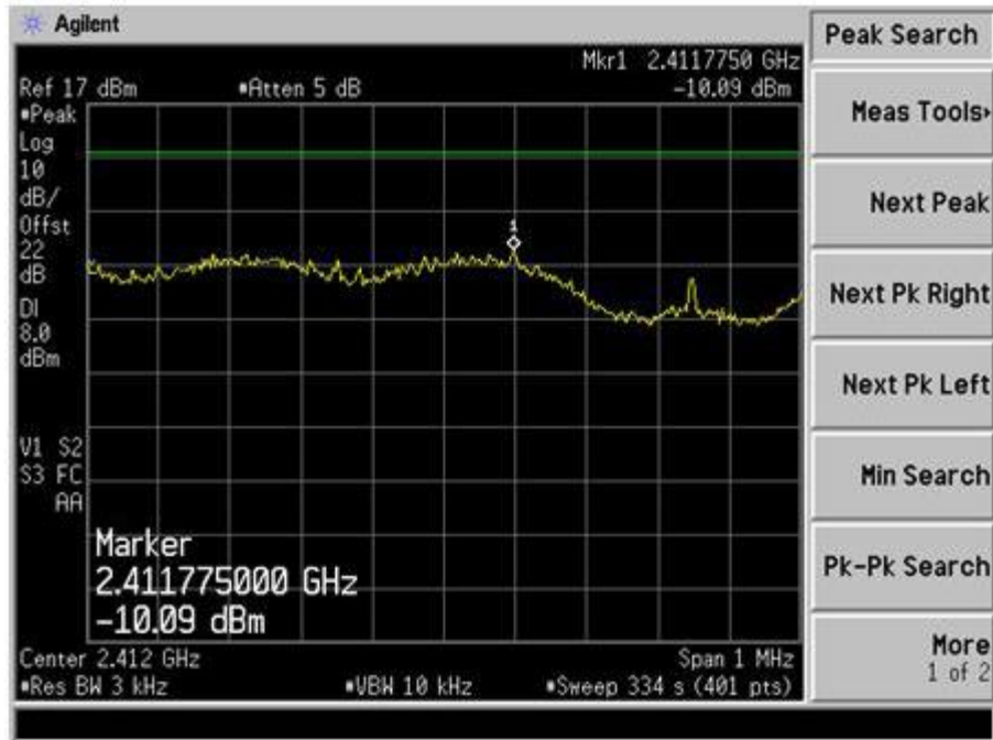
Plot 107 – Channel 1 @ BPSK 9Mbps
