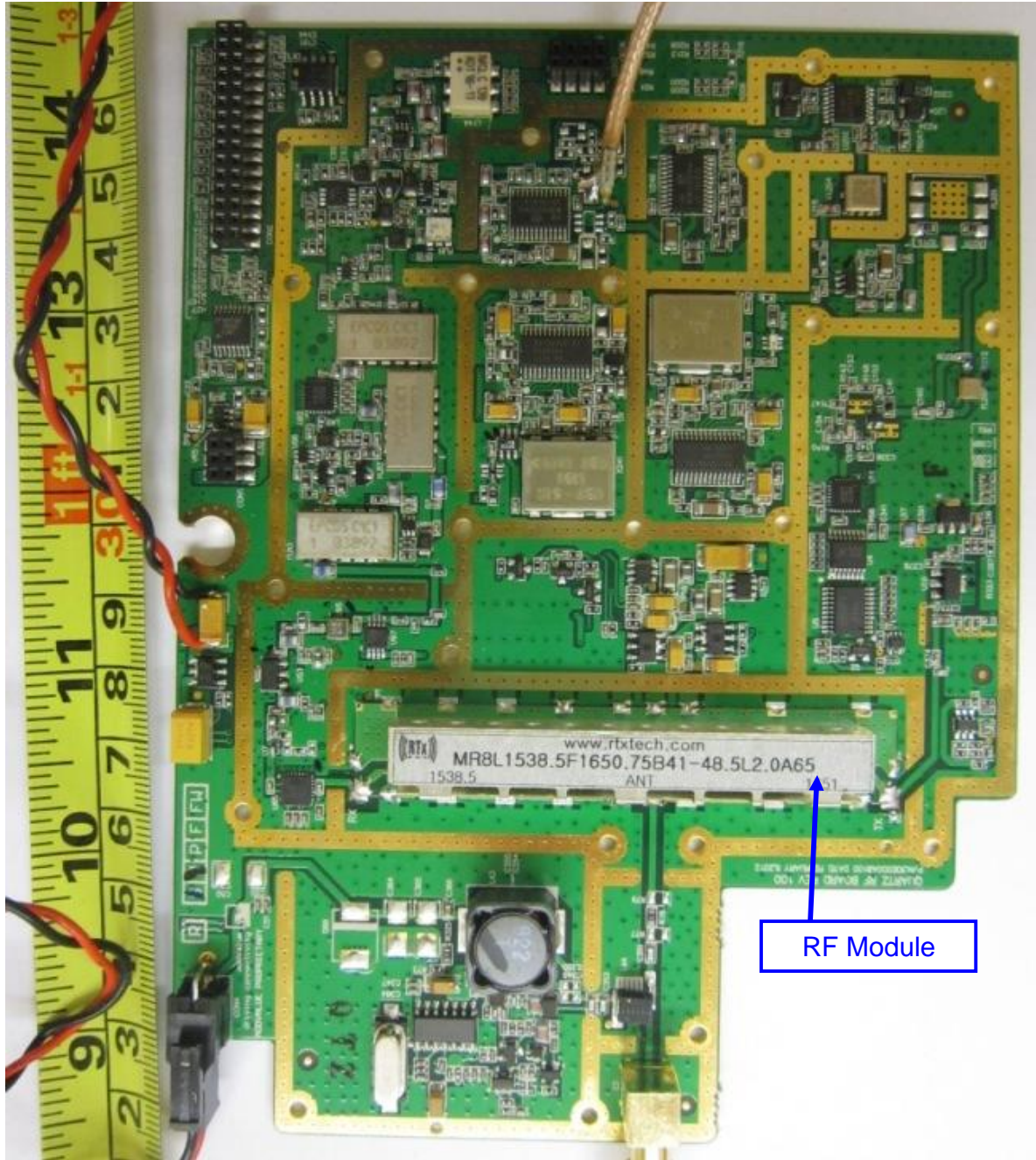
RF Module PCB Component Side
