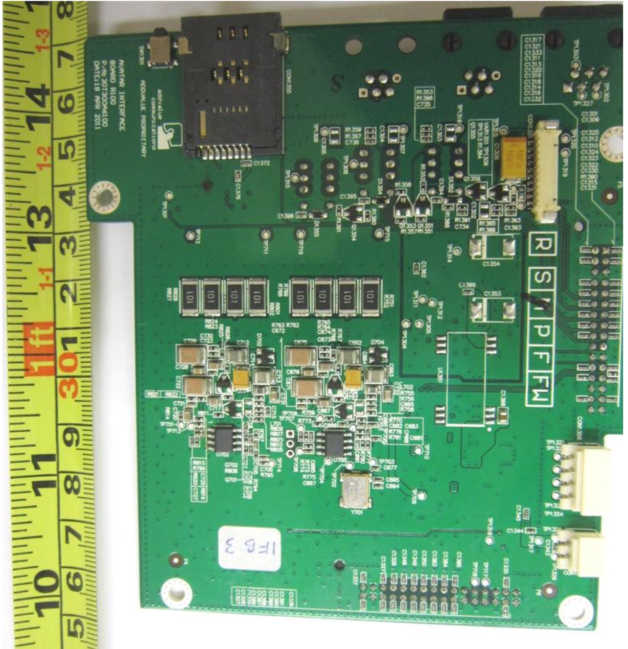
Interface Board PCB Trace Side
