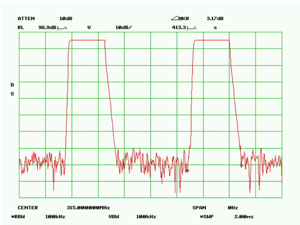
Figure b1: The Pulse width of narrow pulse. Pulse width =0.413ms
