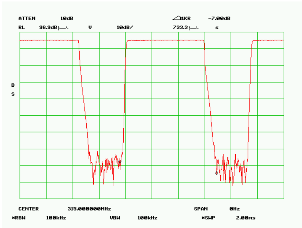
Figure b2: The Pulse width of wide pulse. Pulse width =0.733ms
