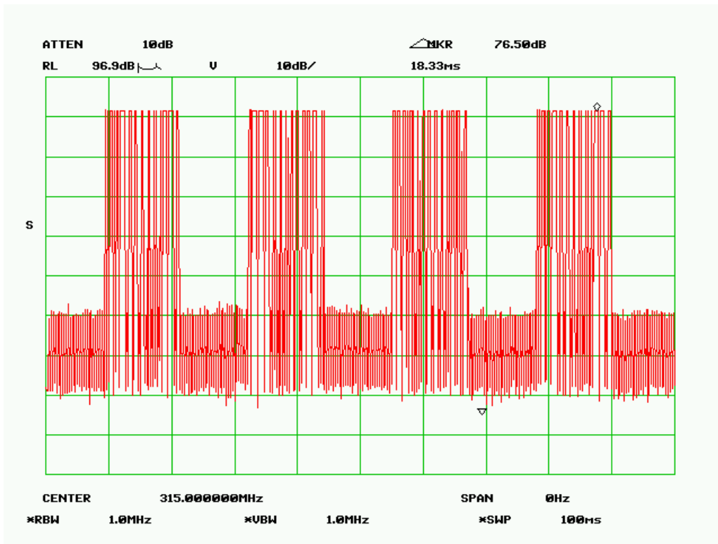
Figure a: The Pulse transmission pattern in 100ms sweep time. (Total of 38 wide pulses and 25 narrow pulses)
