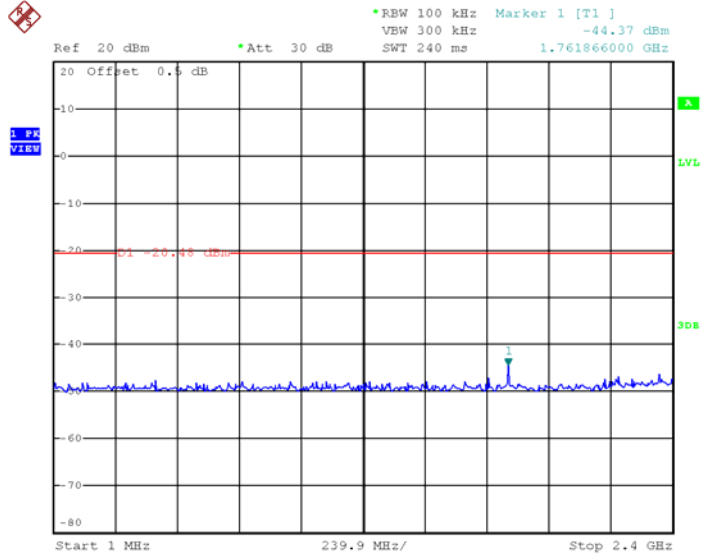
802.11g, Highest Channel, Plot A
