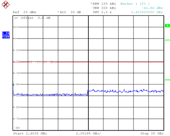
802.11g, Highest Channel, Plot B
