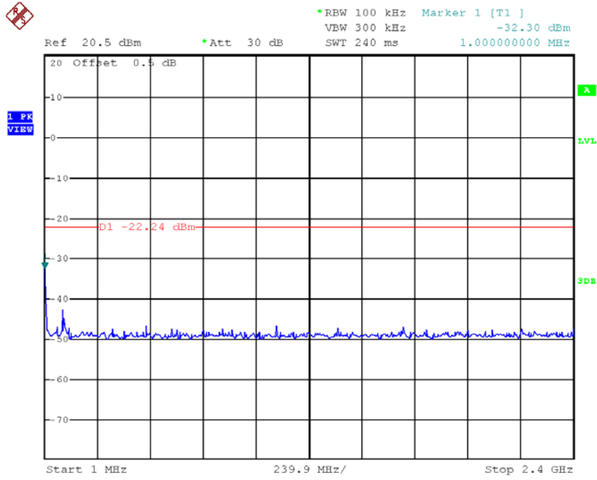
802.11b, Lowest Channel, Plot A
