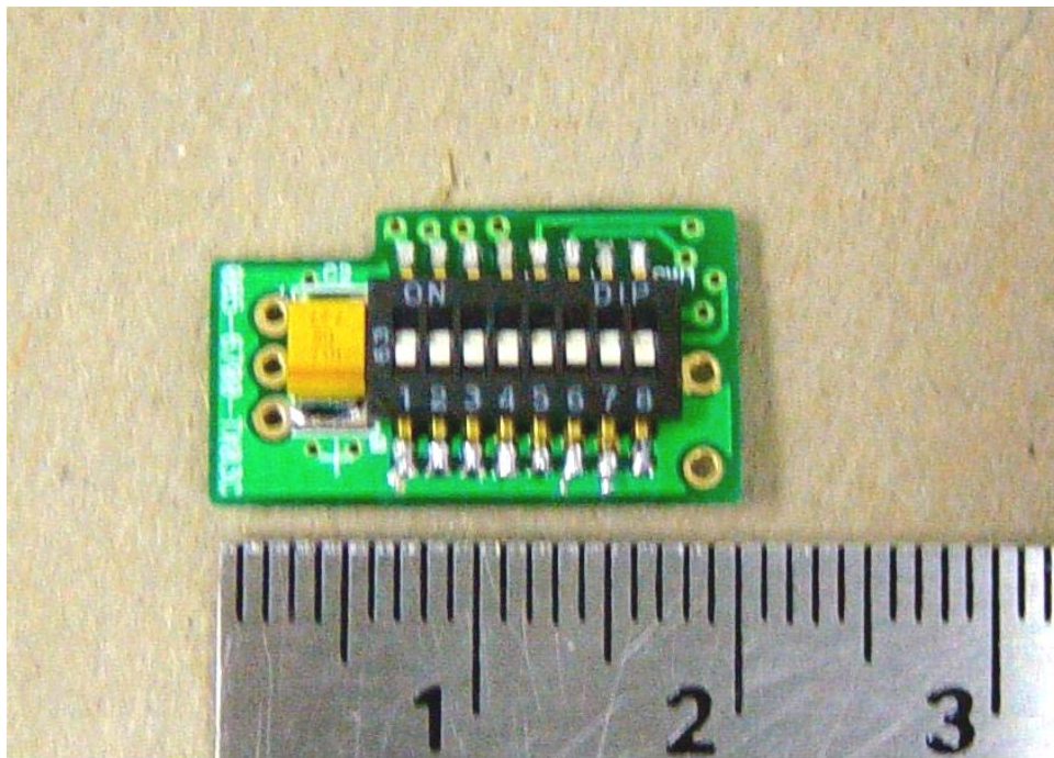
EUT – Board 2 Top Component View
