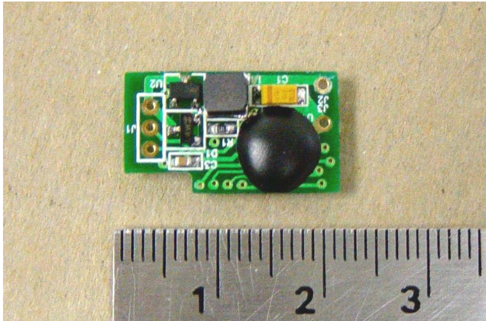
EUT – Board 2 Bottom Component View
