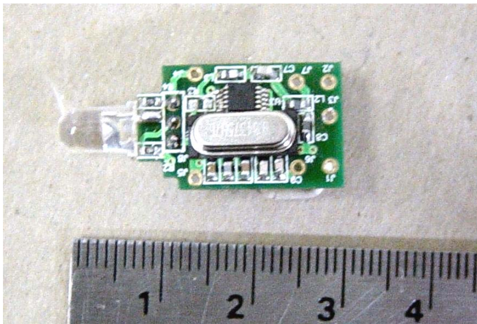
EUT – Board 1 Top Component View
