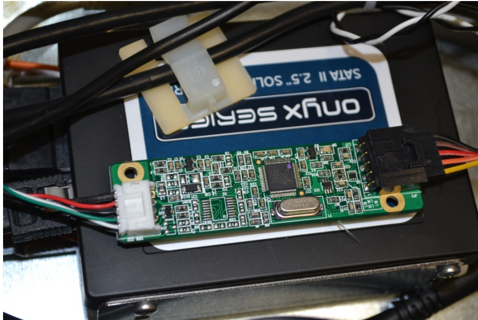
Interface PCB / SSD – Top View
