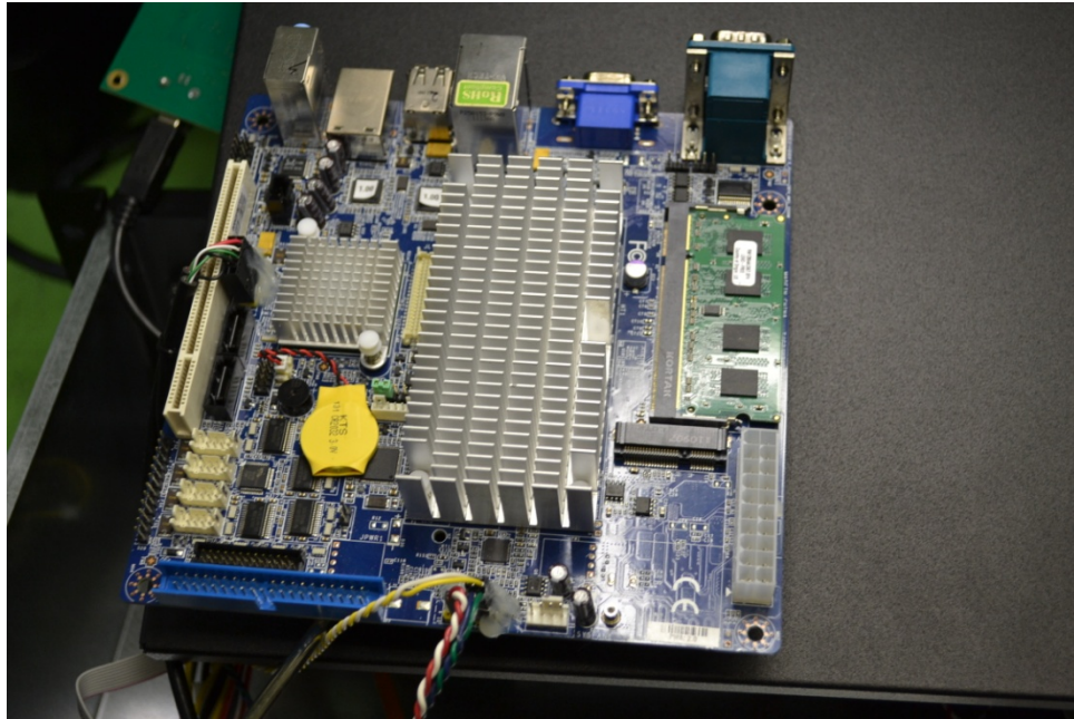
Main PCB – Top Side
