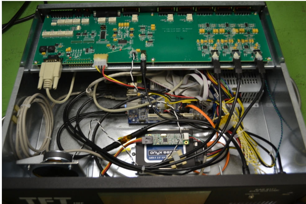
Top Cover Removed
