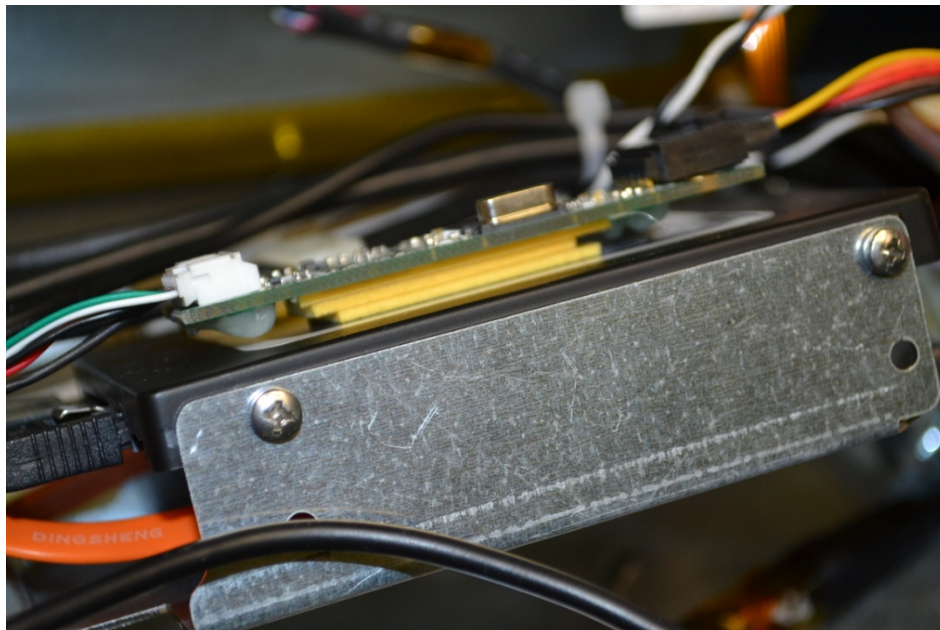
Interface PCB Mounting
