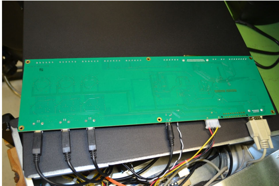
I/O PCB – Solder Side
